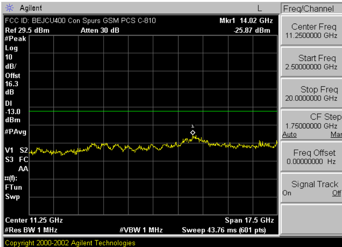
Plot A-18. Conducted Spurious Plot (PCS GSM Mode – Ch. 810)
