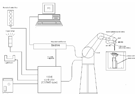
Figure 5-9 SPEAG Robotic System Diagram
