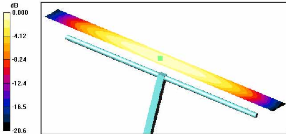
0 dB = 0.500A/m
