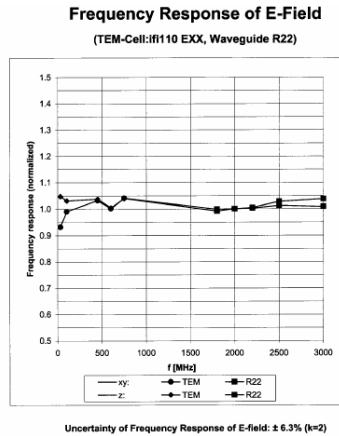
Figure 5-5 E-Field Probe Frequency Response
