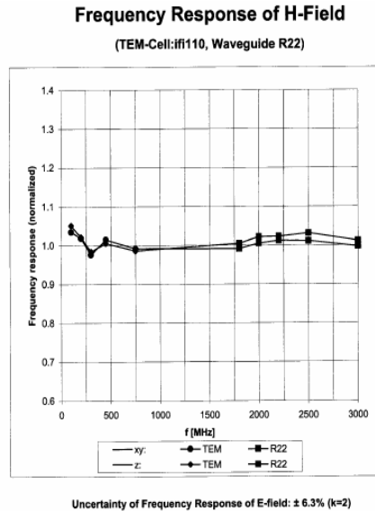
Figure 5-6 H-Field Probe Frequency Response
