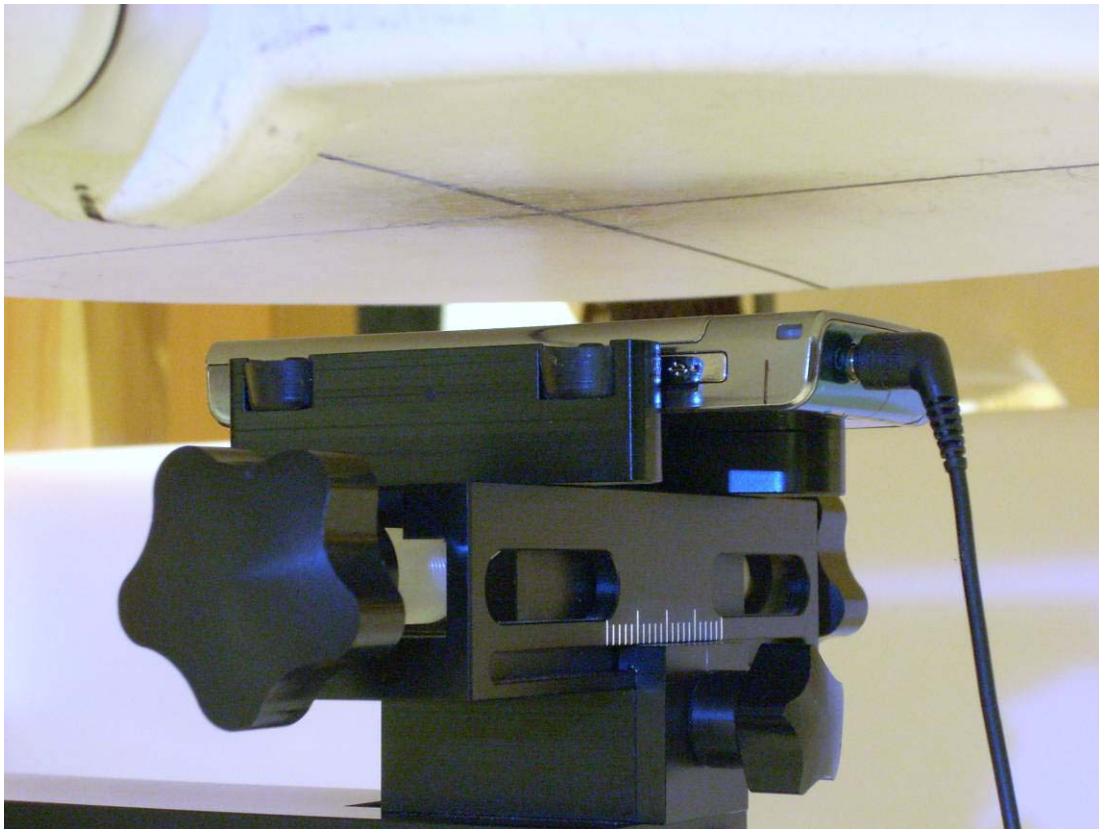
Figure 8: Body SAR, Back Side with 20mm Space
