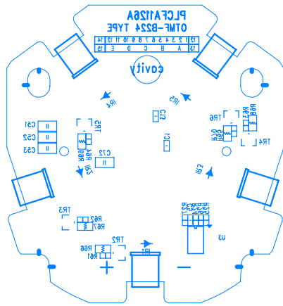
Bottom Silk
