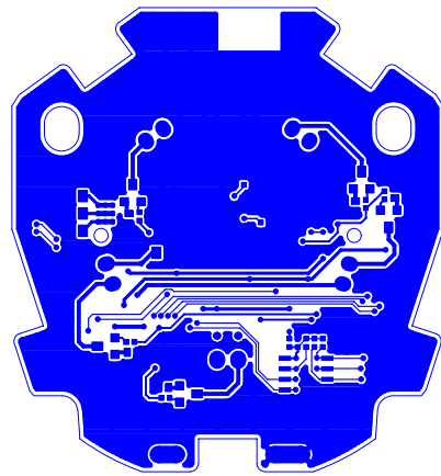
Bottom Pattern
