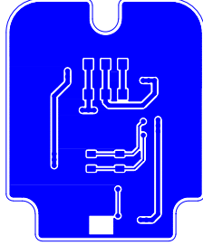
Bottom Pattern
