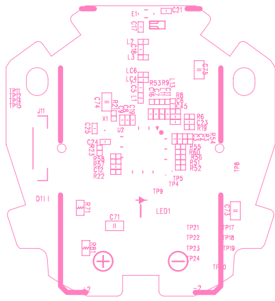
Top Silk
