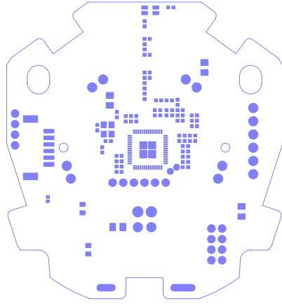
Top Pad
