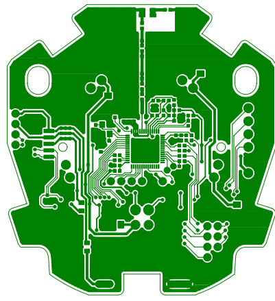
Top Pattern
