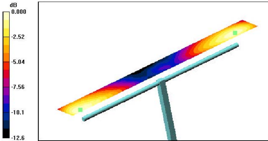
0 dB = 163.5V/m
