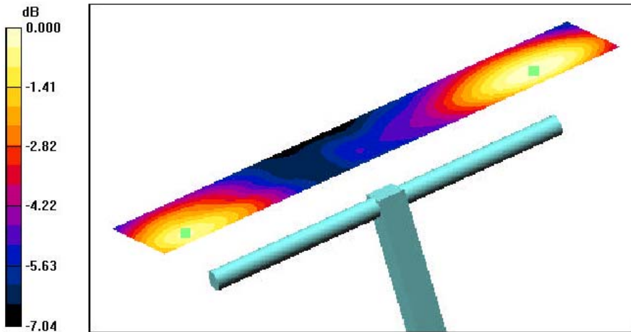
0 dB = 136.7V/m
