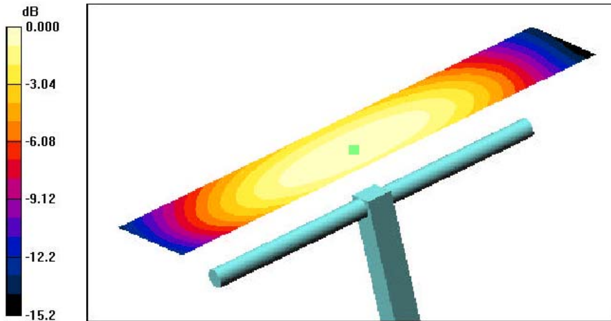
0 dB = 0.446A/m
