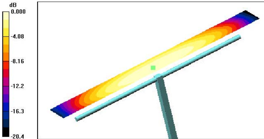
0 dB = 0.421 A/m
