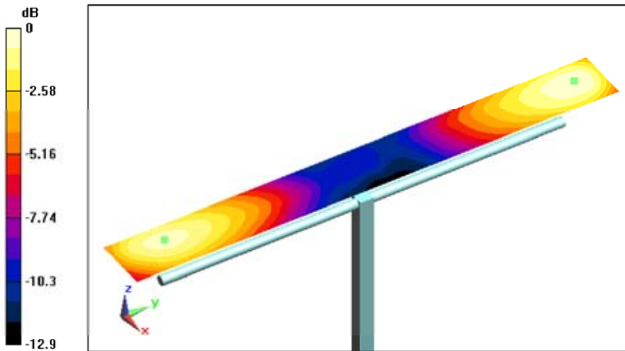
0 dB = 165.1V/m
