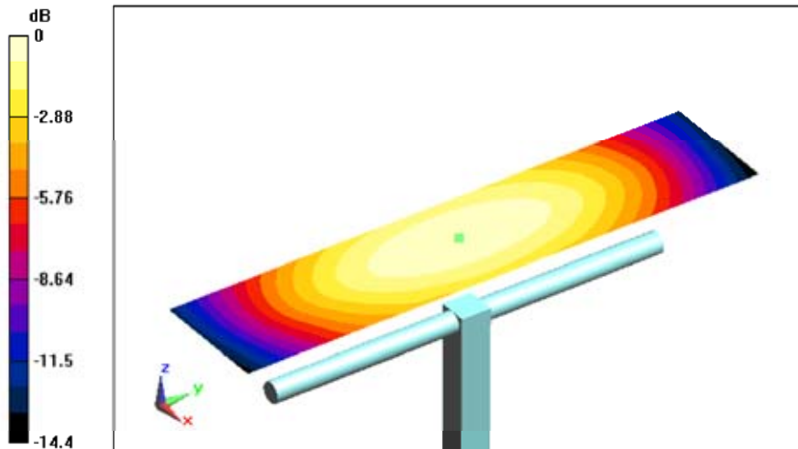
0 dB = 0.419A/m
