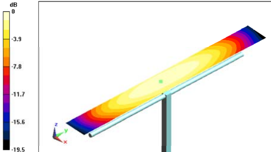
0 dB = 0.408A/m
