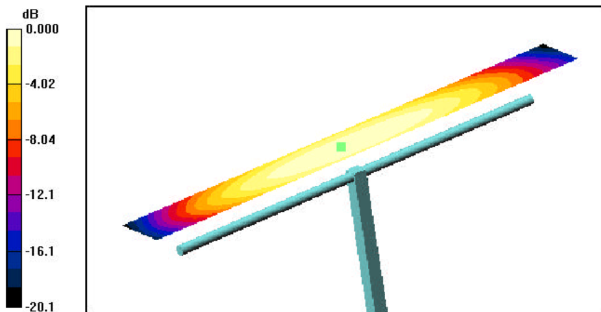
0 dB = 0.461A/m
