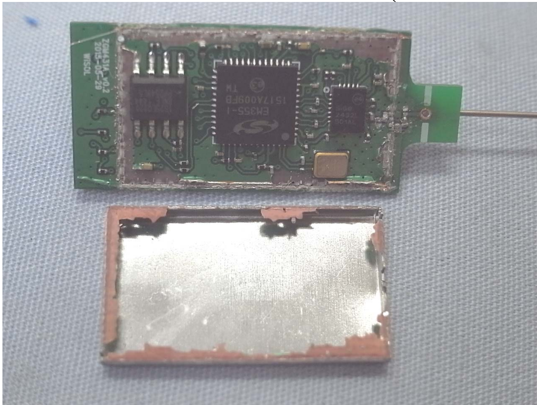
Figure 3 Internal View (Removed Shielded Cover)
