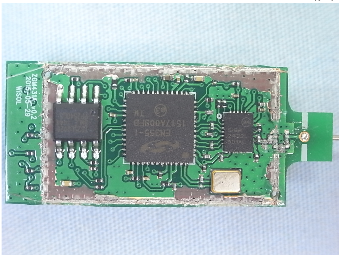
Figure 4 Internal View
