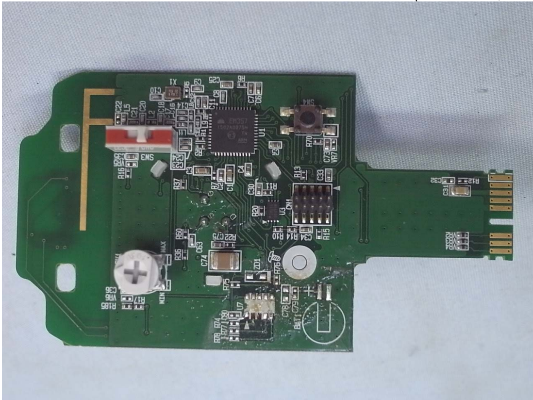
Figure 3 Internal View (Main Board, Front View)
