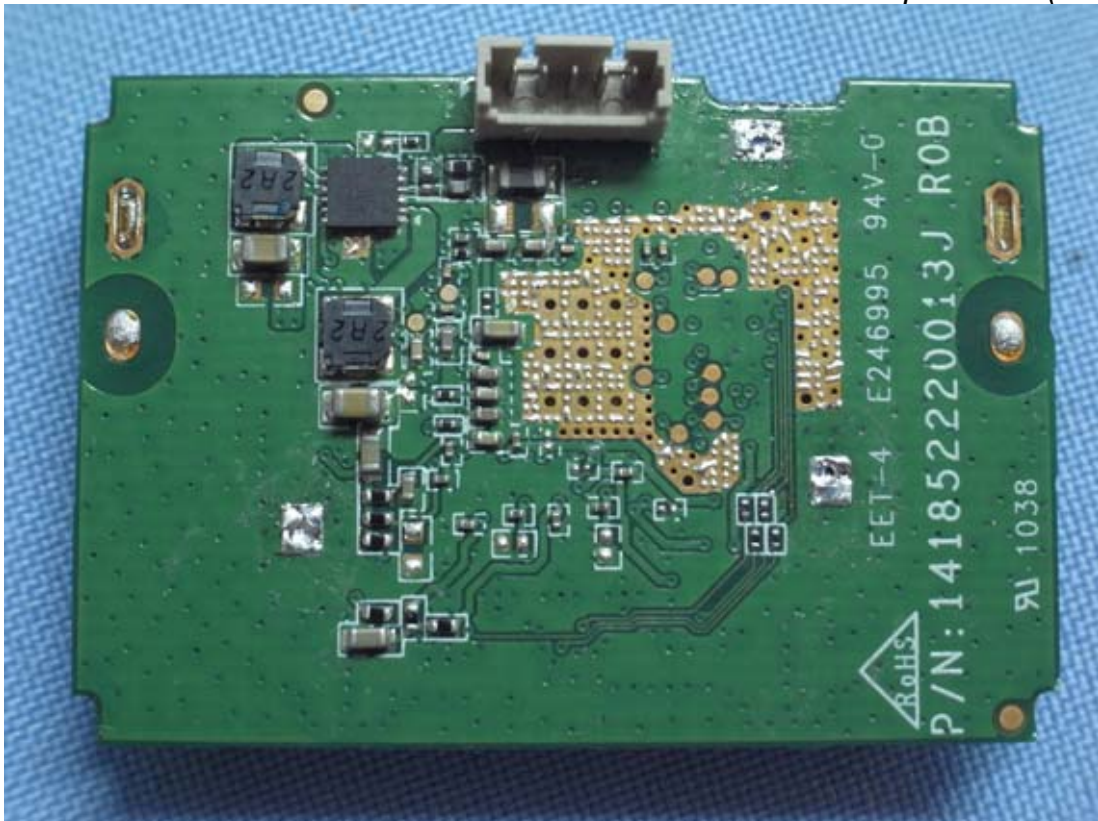
Figure 4 WLAN Adapter Card (Back View)
