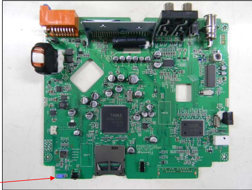
Top view of main board
