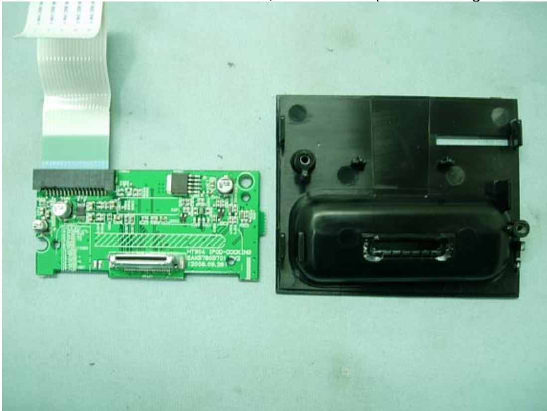
Figure 31 M/N HW904PA, Internal View (IPOD Docking Board Removed)
