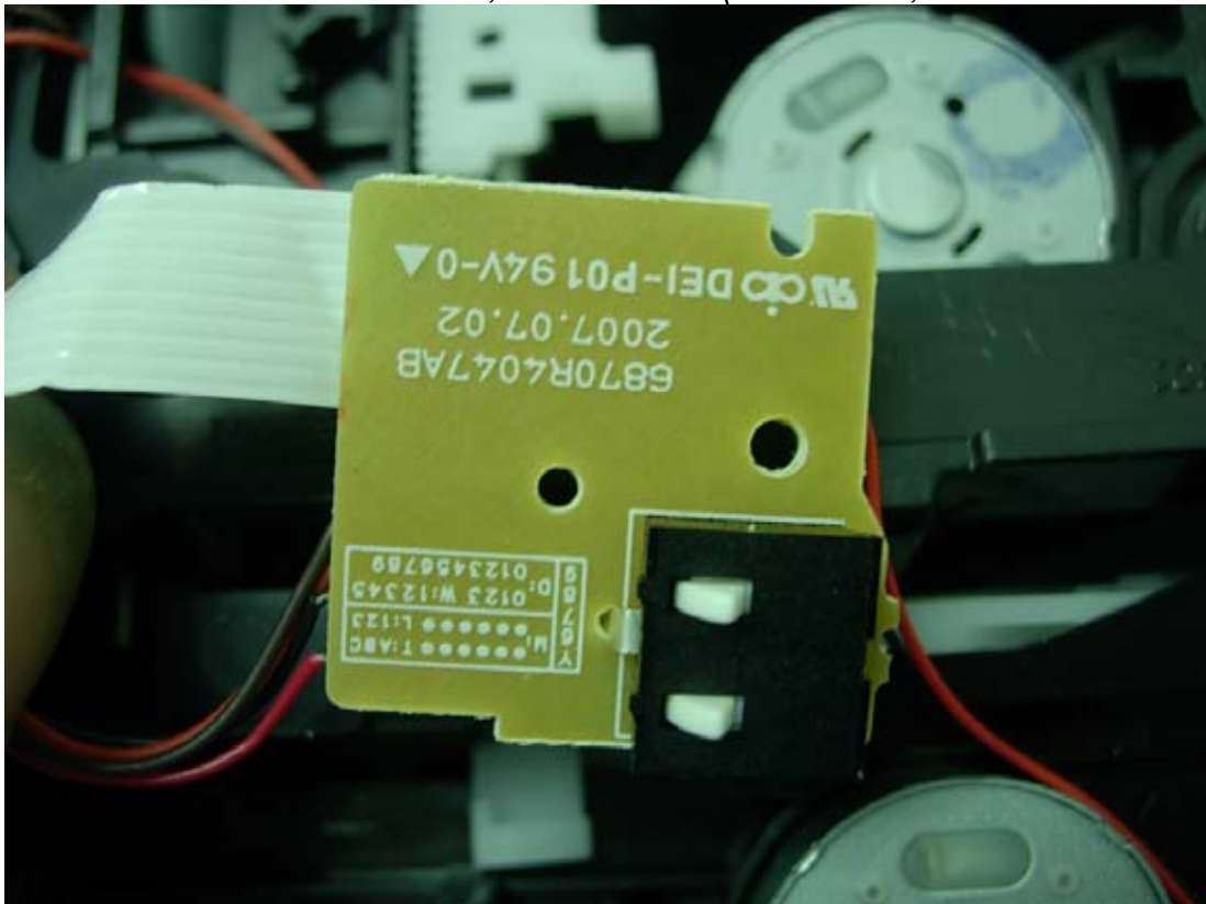
Figure 22 M/N HW904PA, Internal View (DVD Driver, Control Board/Front View)
