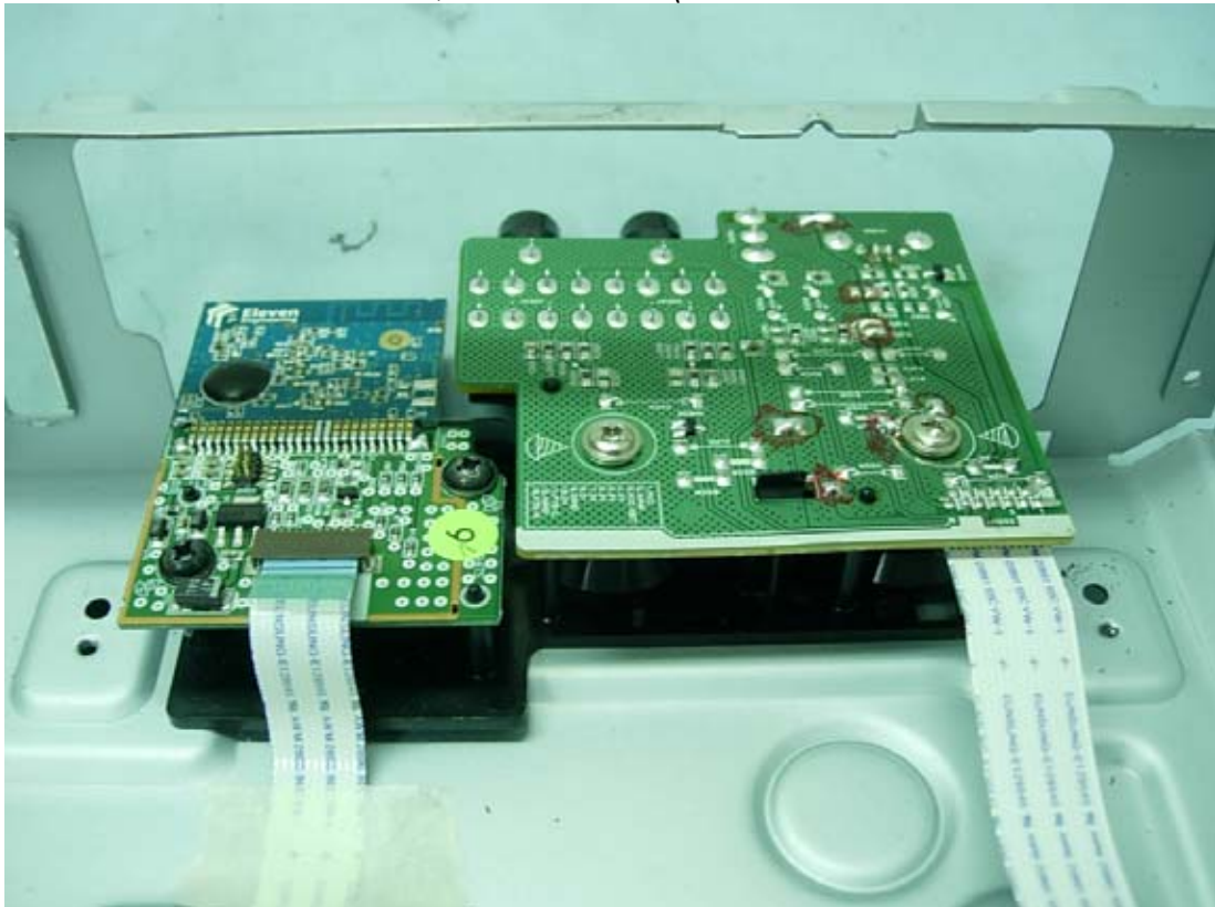
Figure 34 M/N HW904PA, Internal View (RF Module Board & USB/PTB/MIC Board)
