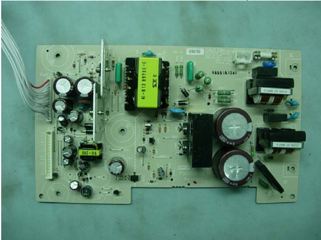
Figure 13 M/N HW904PA, Internal View (Power Board, Front View)
