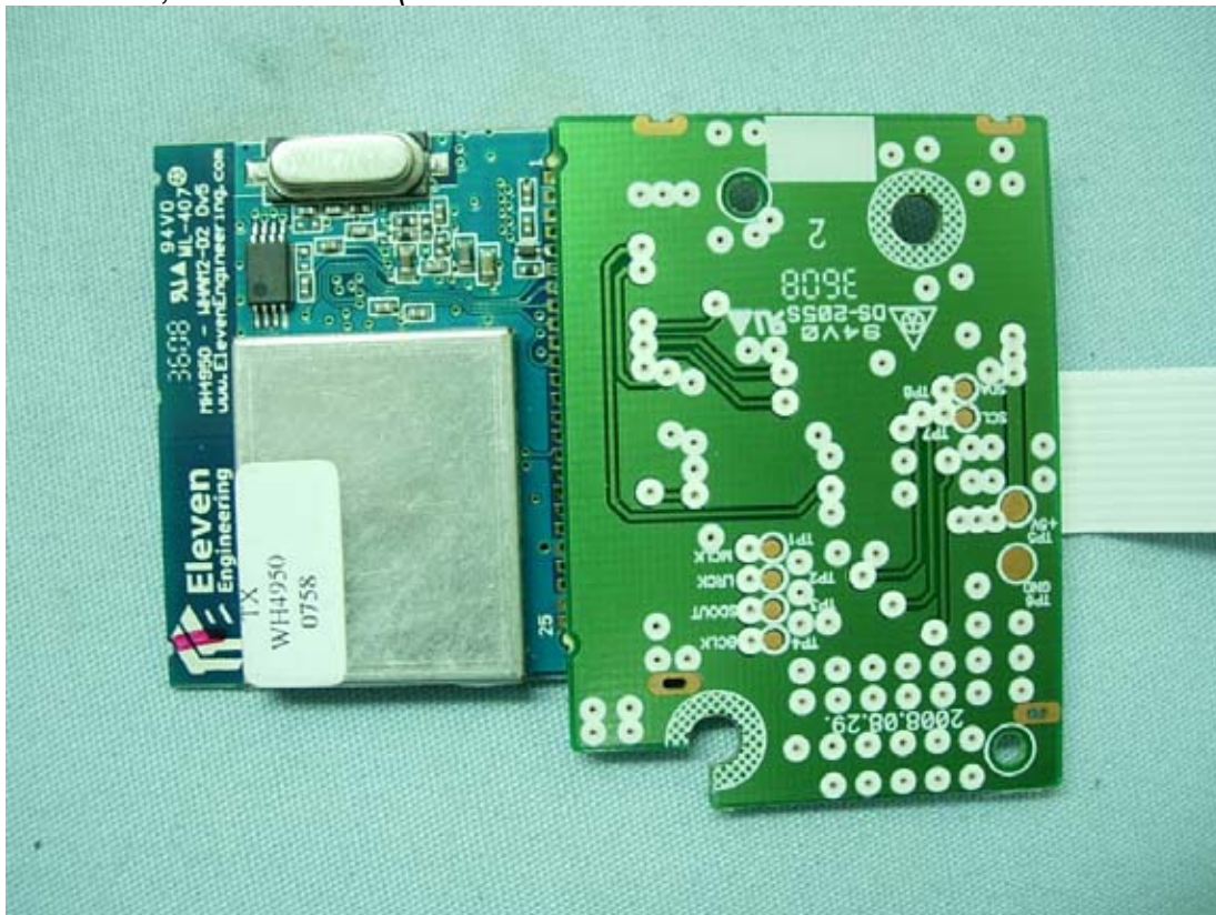
Figure 65 M/N HW964TZ, Internal View (RF Module Board/Front View and Control Board/Back View)
