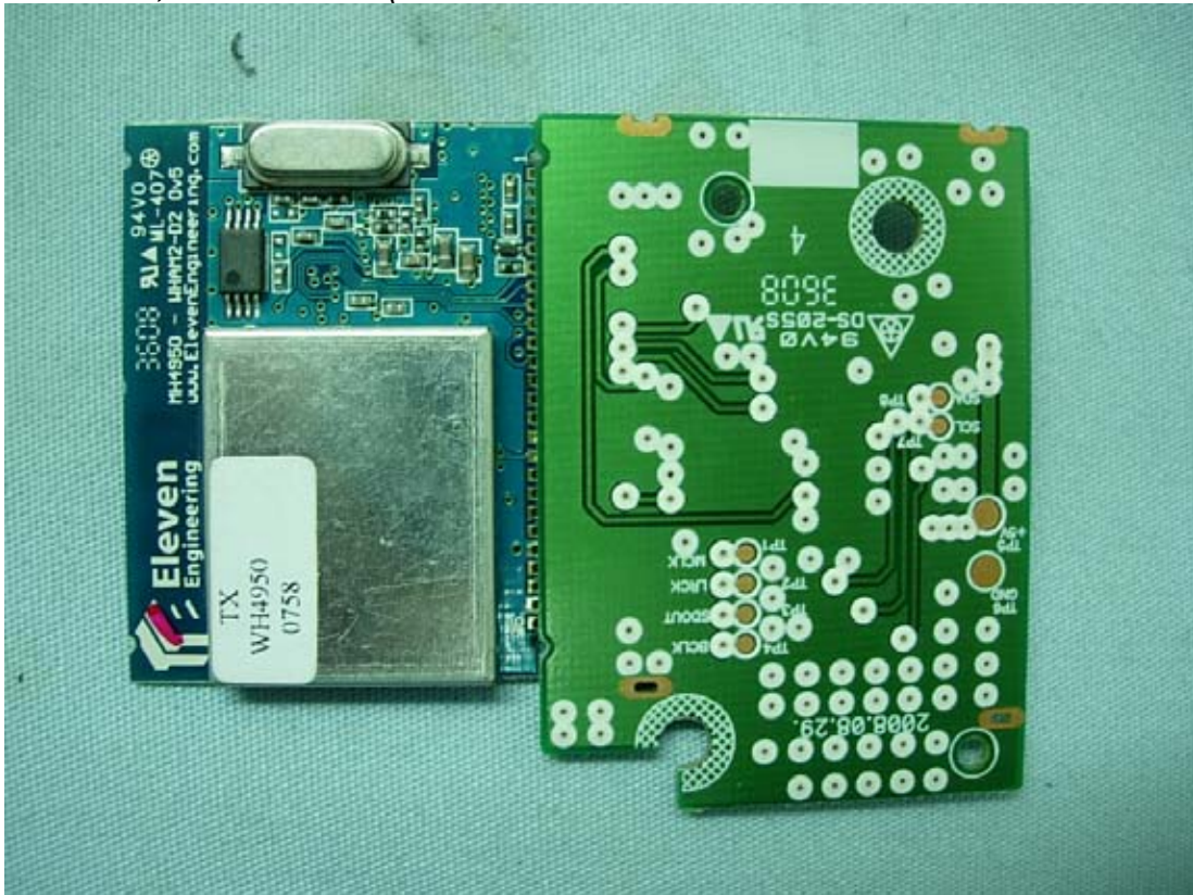
M/N HW904PA, Internal View (RF Module Board/Front View and Control Board/Back View)
