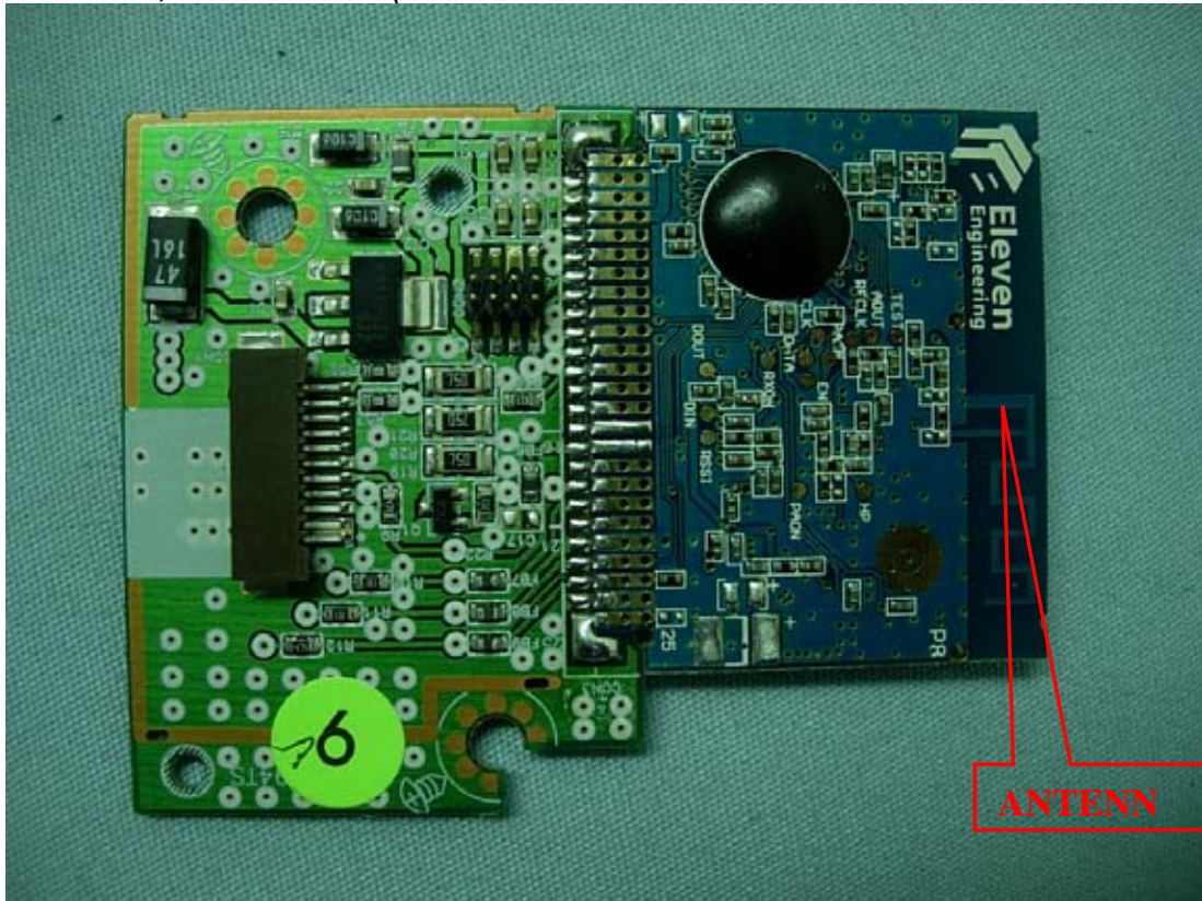
Figure 39 M/N HW904PA, Internal View (RF Module Board/Back View and Control Board/Front View)
