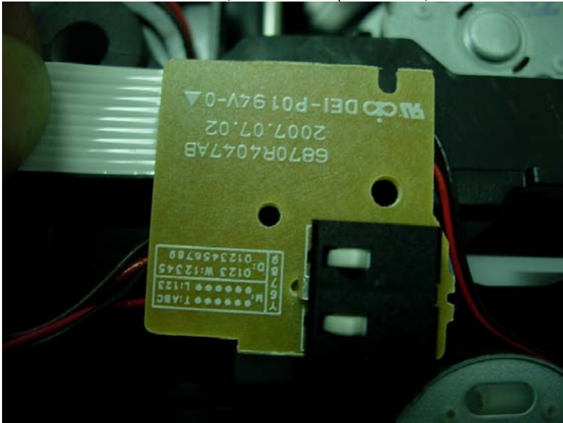
Figure 53 M/N HW964TZ, Internal View (DVD Driver, Control Board/Front View)
