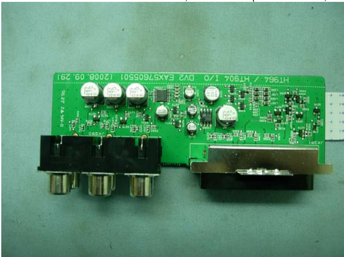
Figure 42 M/N HW964TZ, Internal View (I/O Ports Board, Front View)
