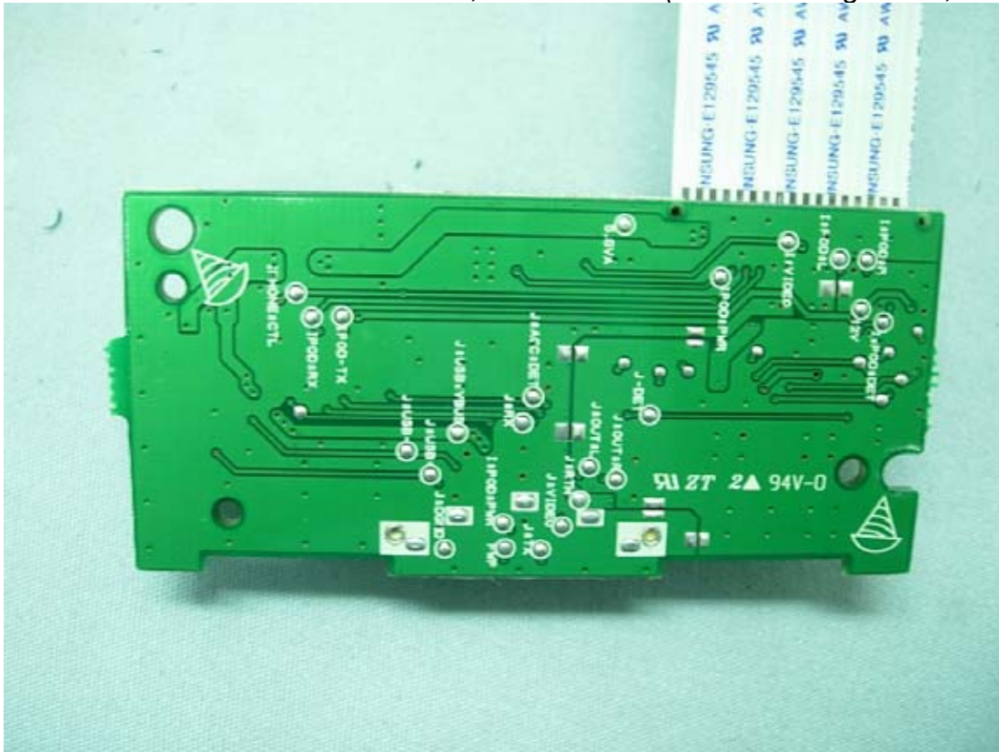
Figure 33 M/N HW904PA, Internal View (IPOD-Docking Board, Back View)
