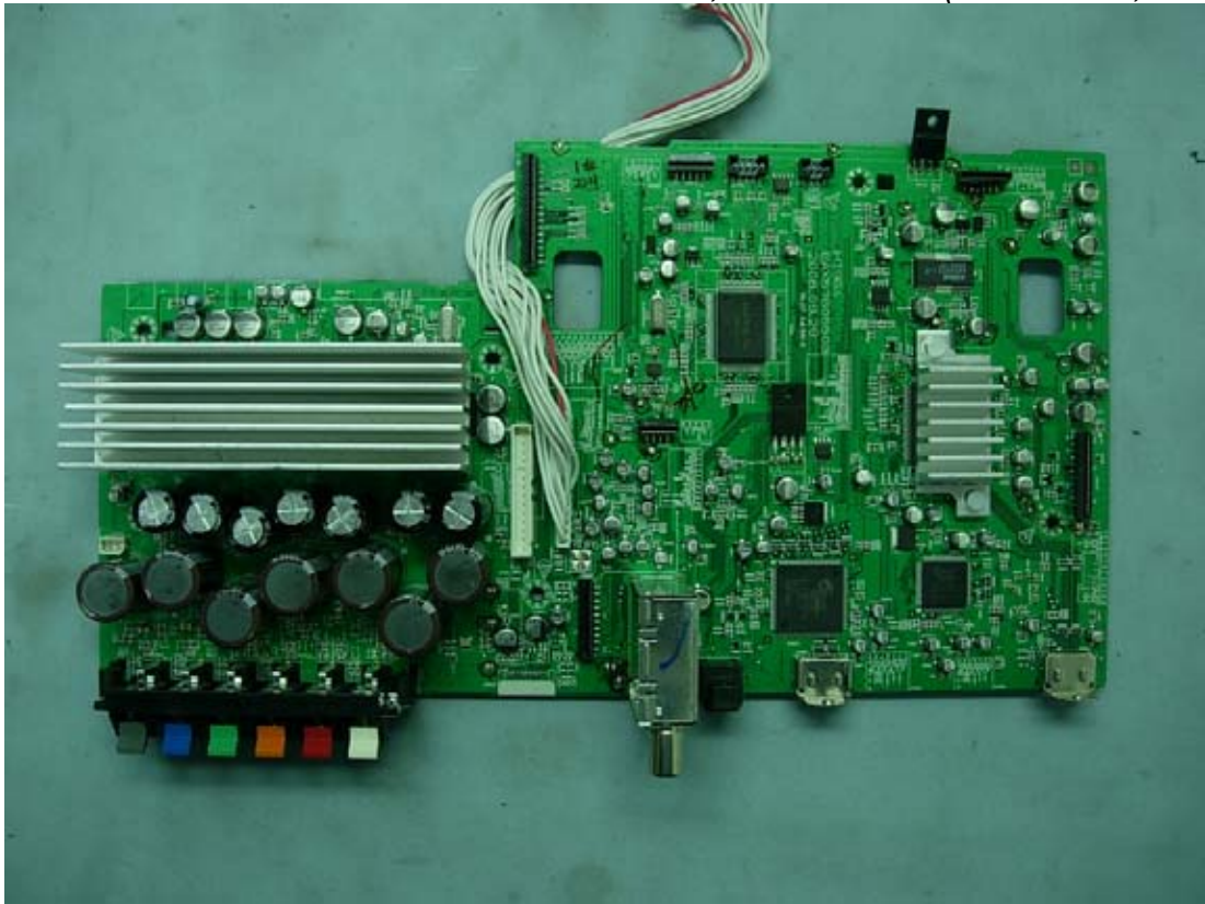
Figure 15 M/N HW904PA, Internal View (Main Board, Front View)
