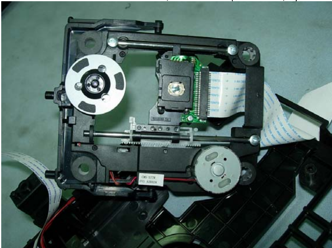
Figure 54 M/N HW964TZ, Internal View (DVD Driver, Optical and Motor)
