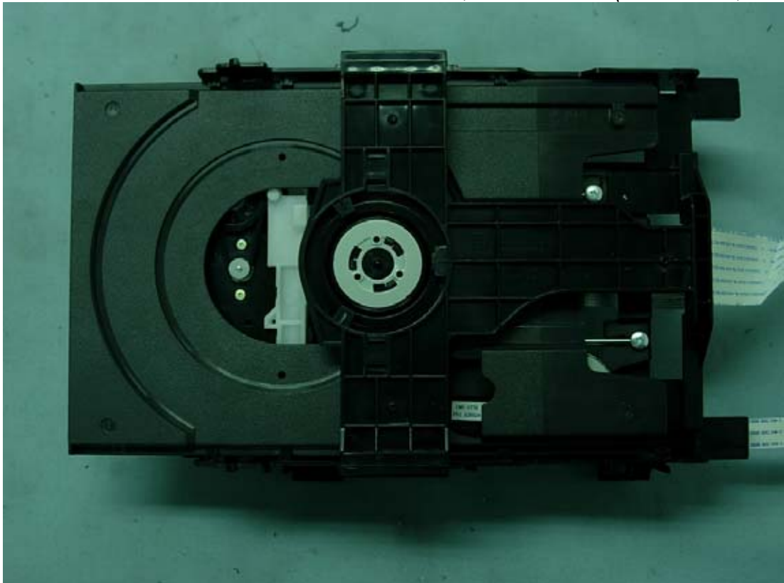
Figure 50 M/N HW964TZ, Internal View (DVD Driver, Front View)
