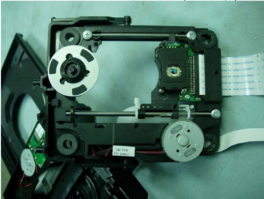
Figure 23 M/N HW904PA, Internal View (DVD Driver, Optical and Motor)
