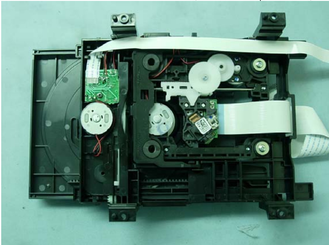
Figure 20 M/N HW904PA, Internal View (DVD Driver, Back View)
