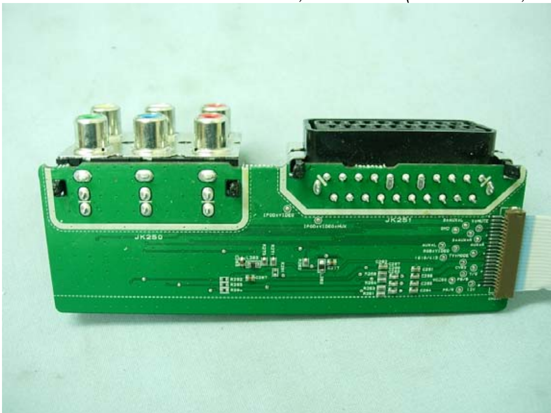
Figure 12 M/N HW904PA, Internal View (I/O Ports Board, Back View)
