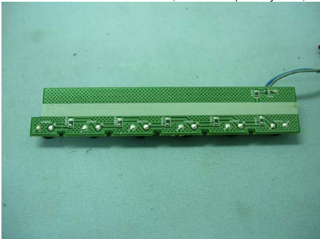
Figure 30 M/N HW904PA, Internal View (Tact-Key Board, Back View)
