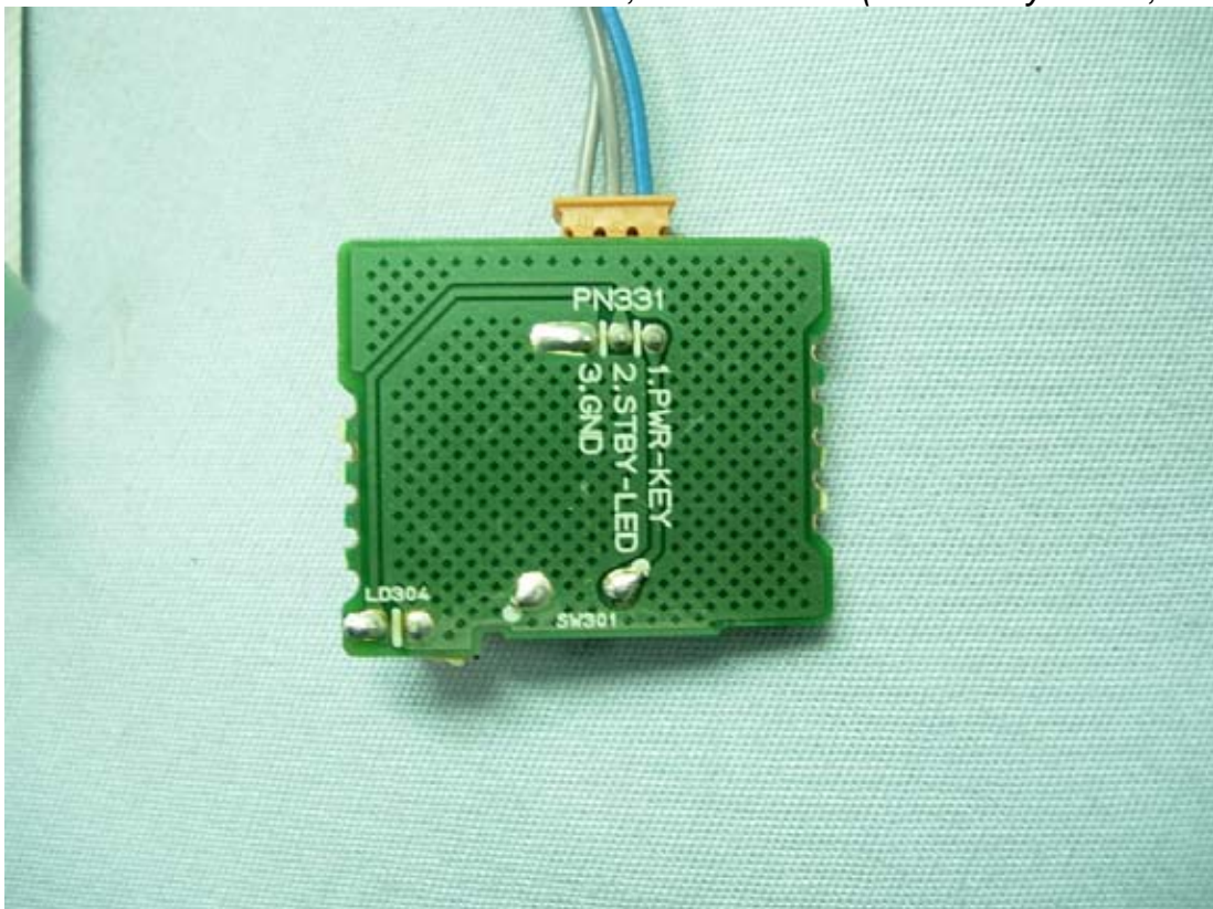
Figure 28 M/N HW904PA, Internal View (Power Key Board, Back View)
