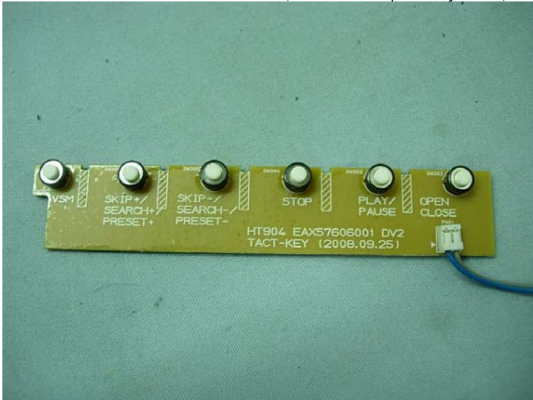
Figure 29 M/N HW904PA, Internal View (Tact-Key Board, Front View)
