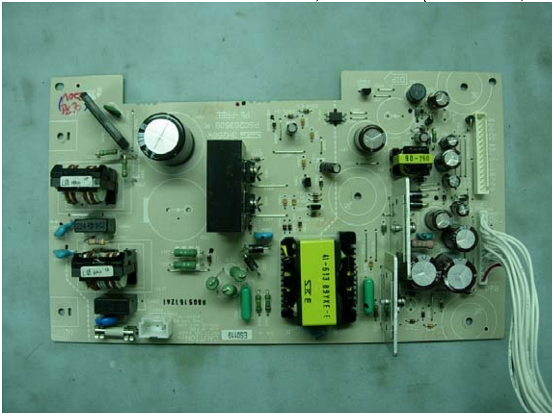
Figure 44 M/N HW964TZ, Internal View (Power Board, Front View)
