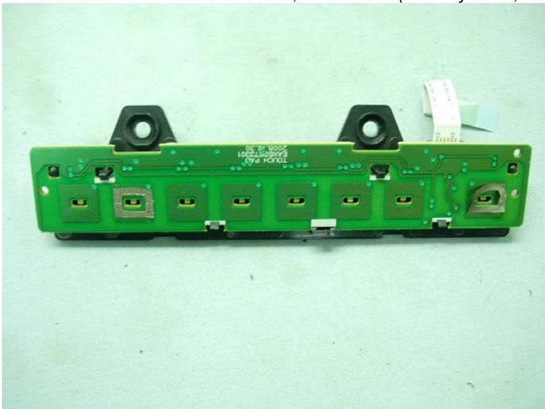
Figure 60 M/N HW964TZ, Internal View (Tact-Key Board, Front View)
