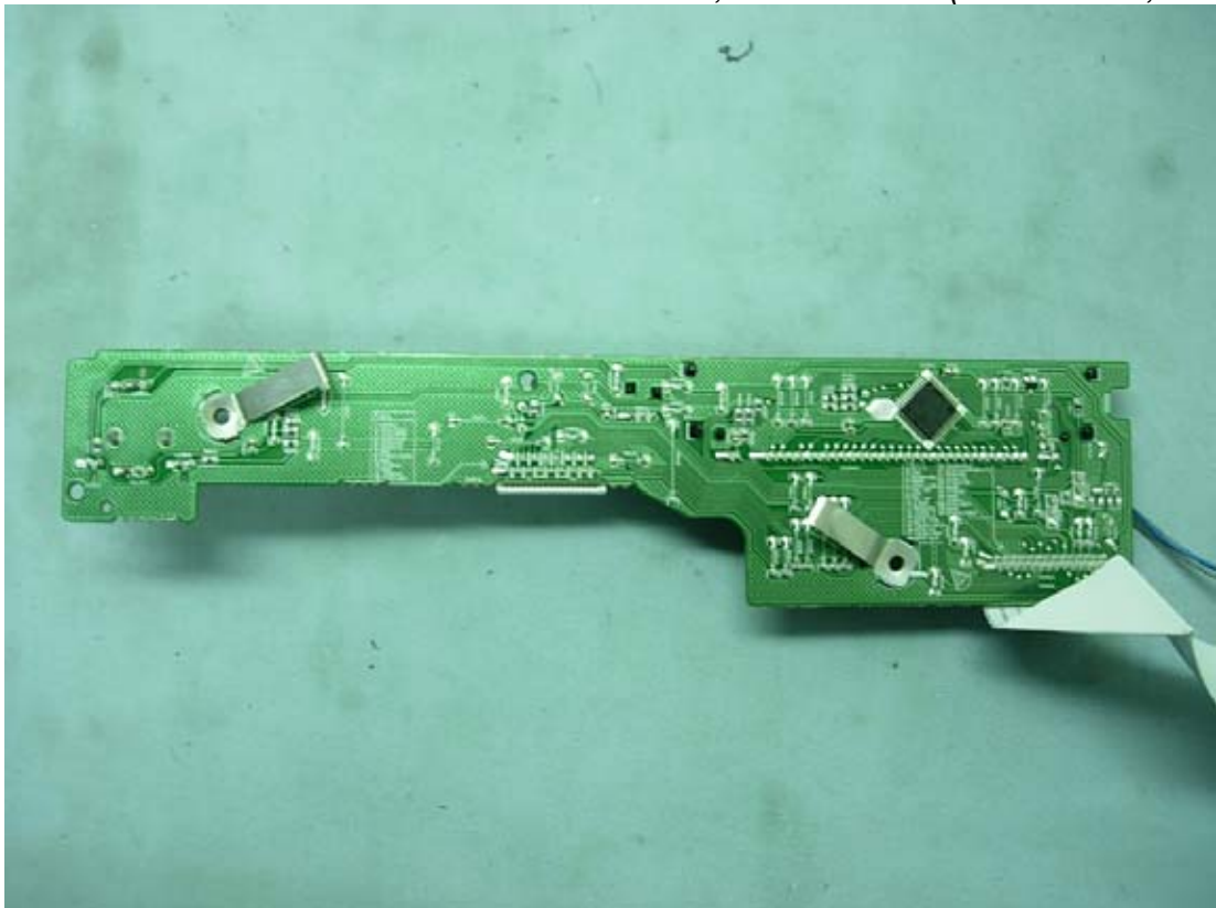
Figure 26 M/N HW904PA, Internal View (Front Board, Back View)
