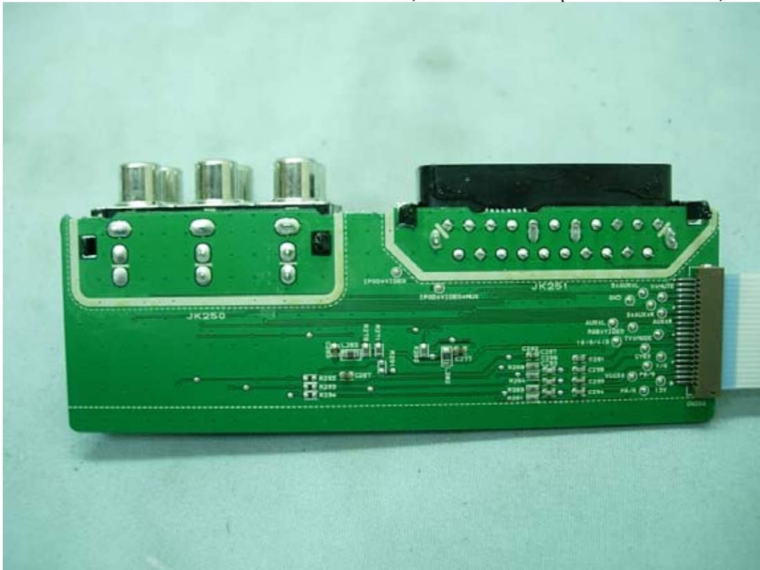
Figure 43 M/N HW964TZ, Internal View (I/O Ports Board, Back View)
