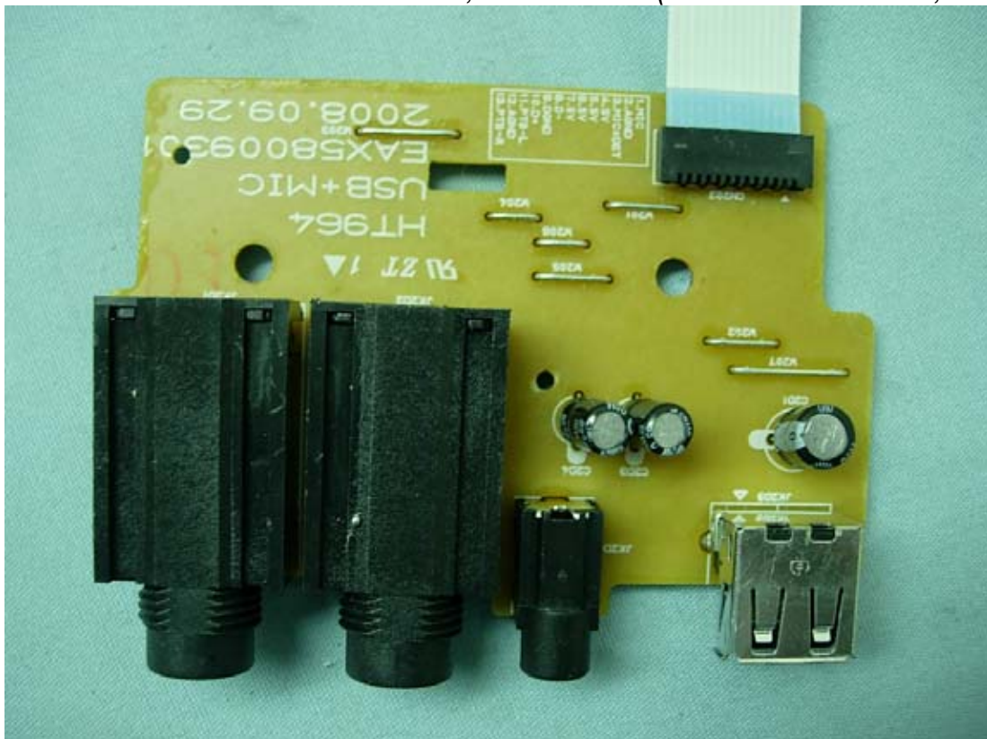
Figure 64 M/N HW964TZ, Internal View (USB/PTB/MIC Board, Back View)
