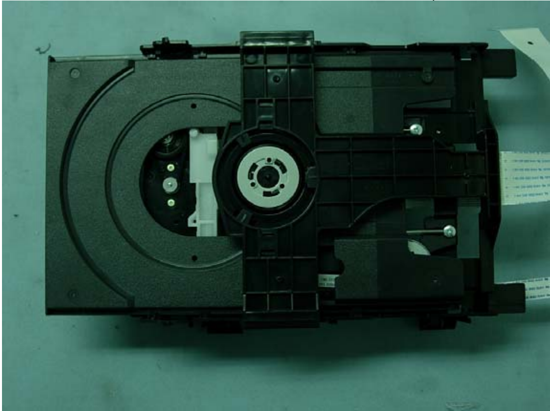
Figure 19 M/N HW904PA, Internal View (DVD Driver, Front View)
