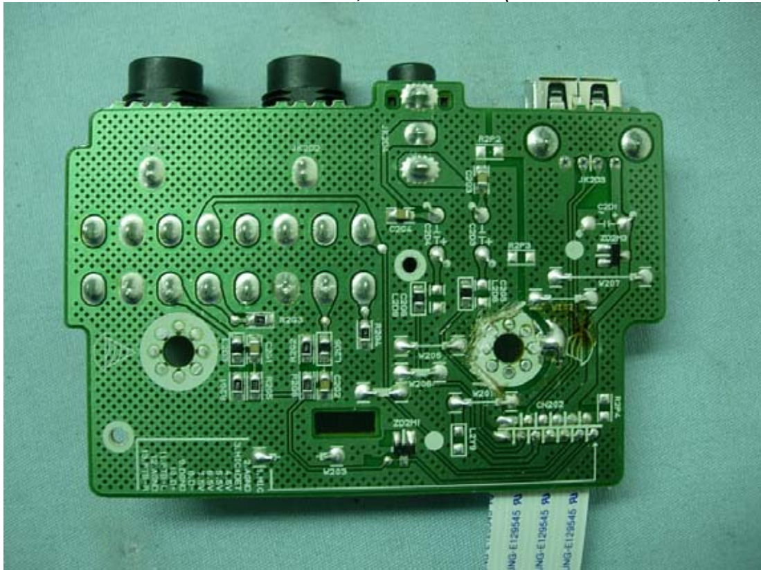
Figure 63 M/N HW964TZ, Internal View (USB/PTB/MIC Board, Front View)
