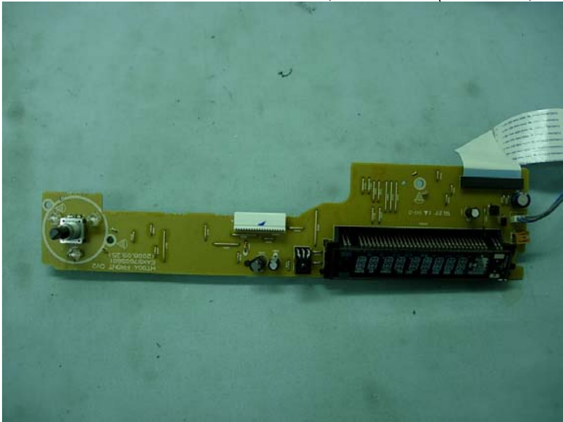
Figure 25 M/N HW904PA, Internal View (Front Board, Front View)
