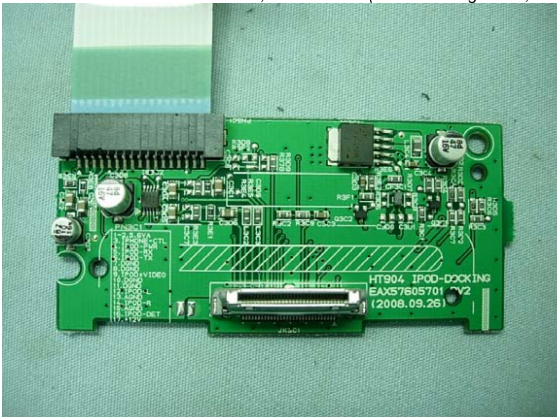
Figure 32 M/N HW904PA, Internal View (IPOD-Docking Board, Front View)
