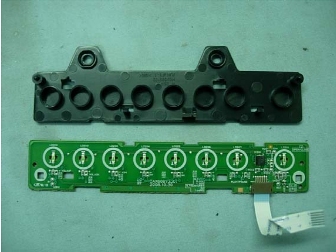
Figure 61 M/N HW964TZ, Internal View (Tact-Key Board, Back View)
