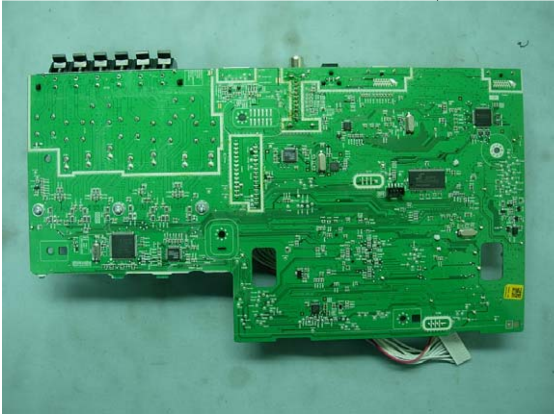
Figure 49 M/N HW964TZ, Internal View (Main Board, Back View)
