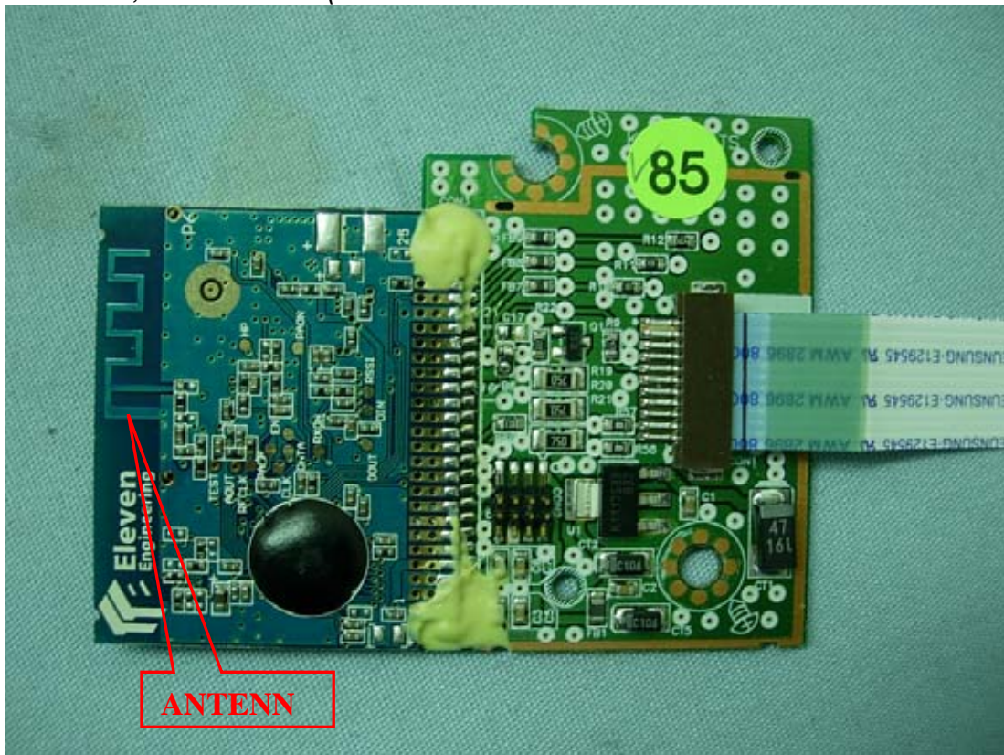
Figure 67 M/N HW964TZ, Internal View (RF Module Board/Back View and Control Board/Front View)
