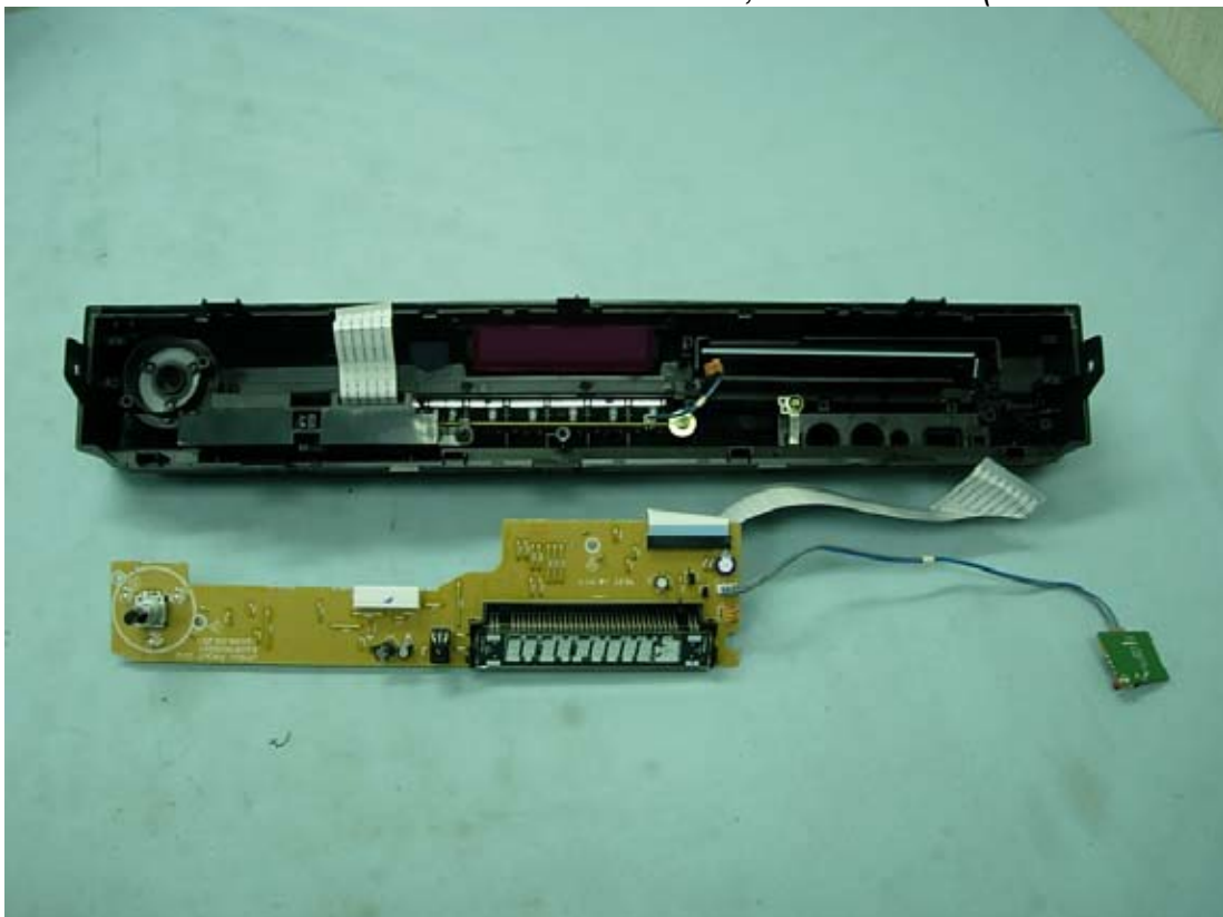
Figure 24 M/N HW904PA, Internal View (Front Board Removed)
