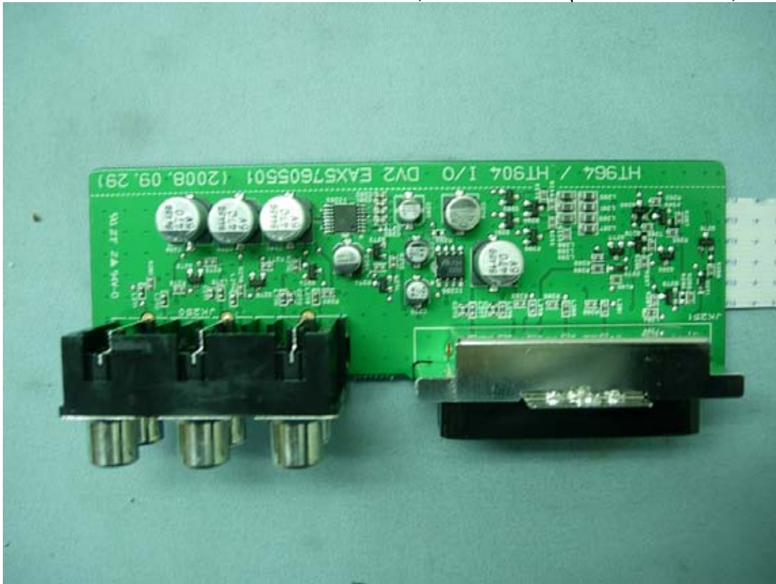
Figure 11 M/N HW904PA, Internal View (I/O Ports Board, Front View)
