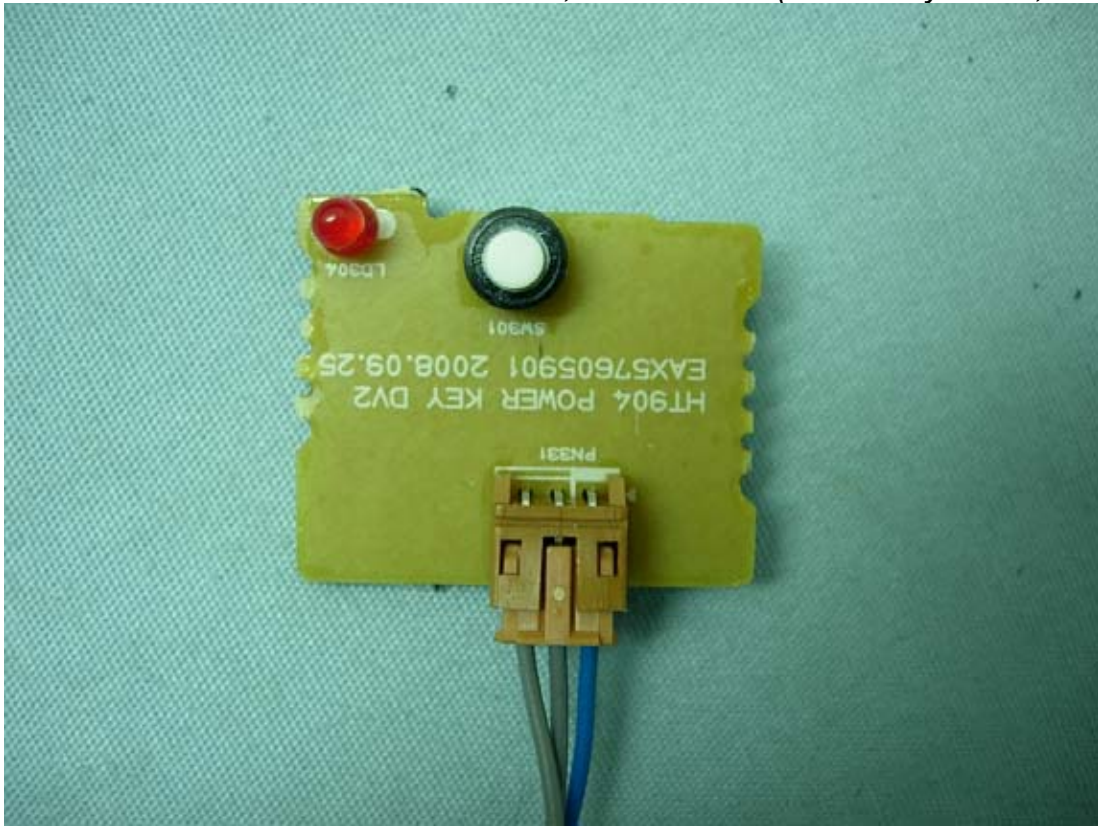
Figure 27 M/N HW904PA, Internal View (Power Key Board, Front View)
