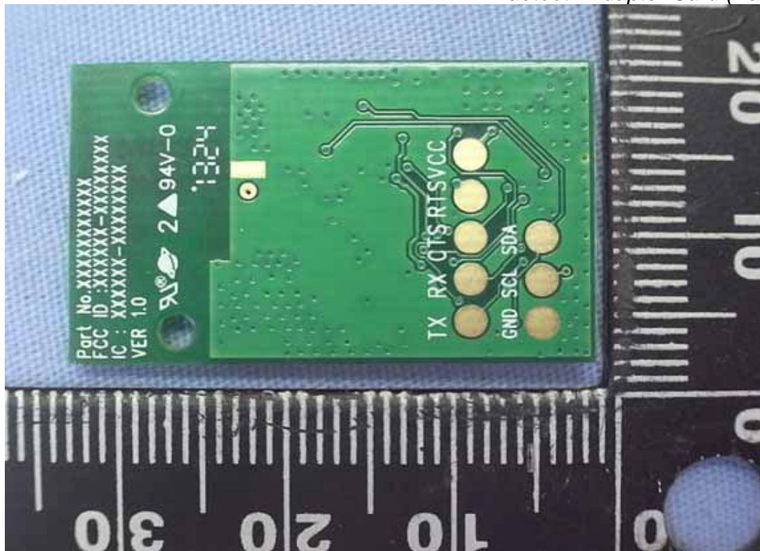
Figure 3 Bluetooth Adapter Card (Back View)
