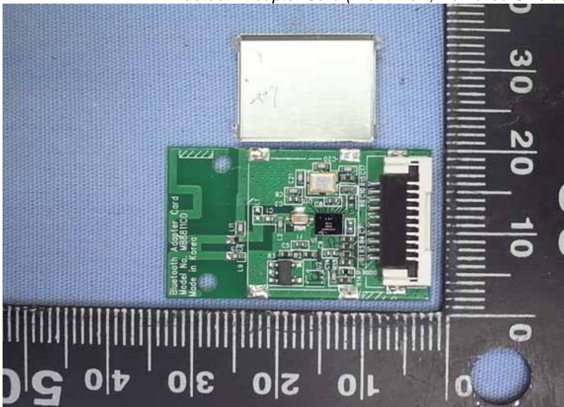
Bluetooth Adapter Card (Front View, Removed Shielded Case)
