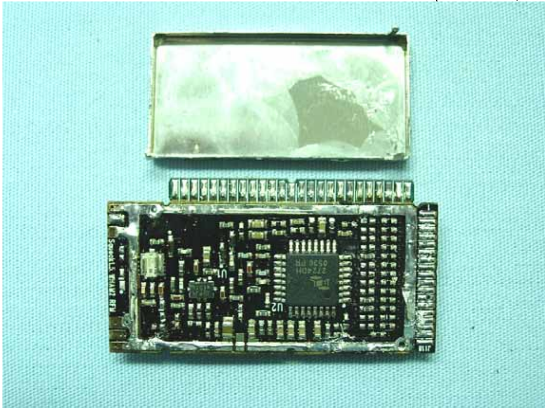
Figure 10 Internal View (TX Module, Back View)
