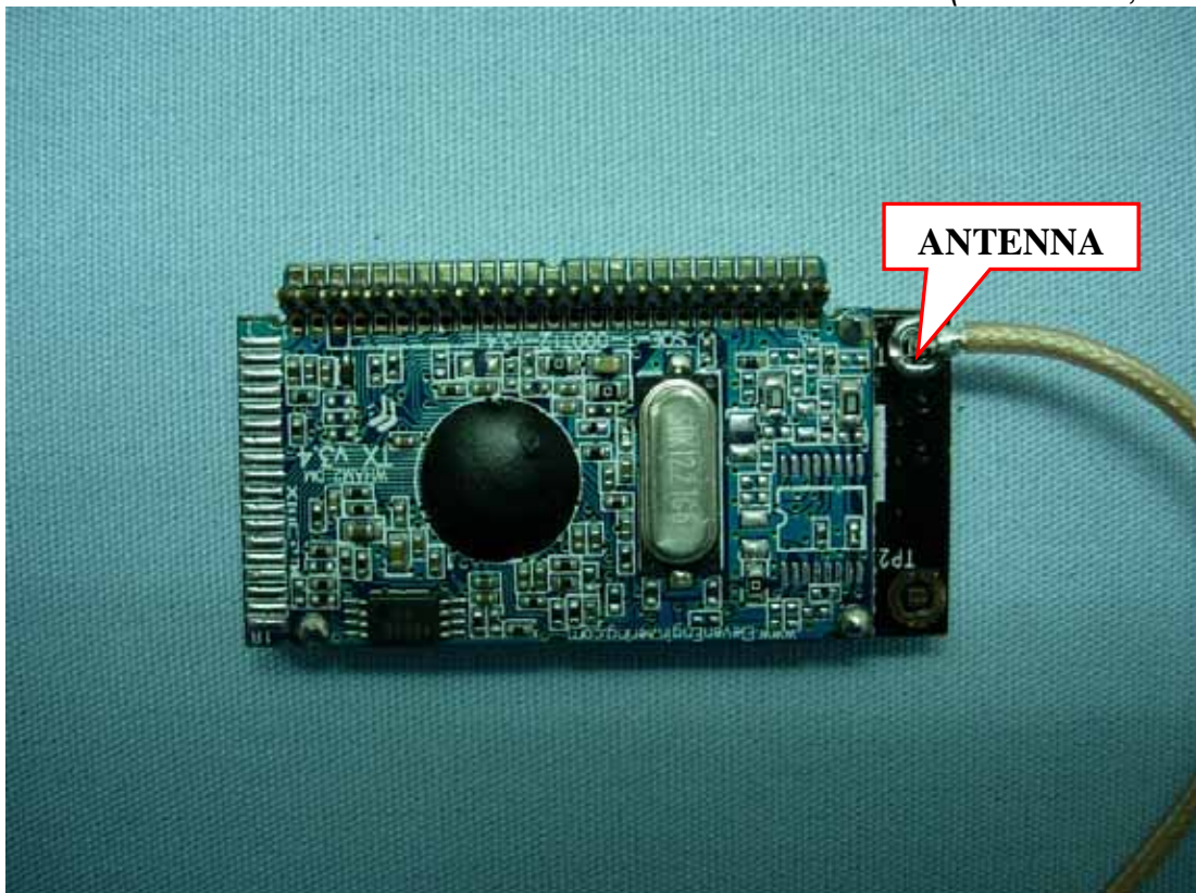
Figure 9 Internal View (TX Module, Front View)
