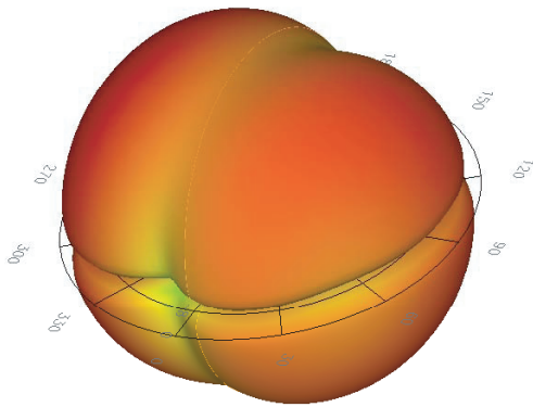
3D Gain Plot
