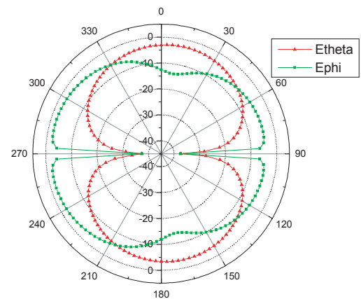
x - z cut (dBi)
