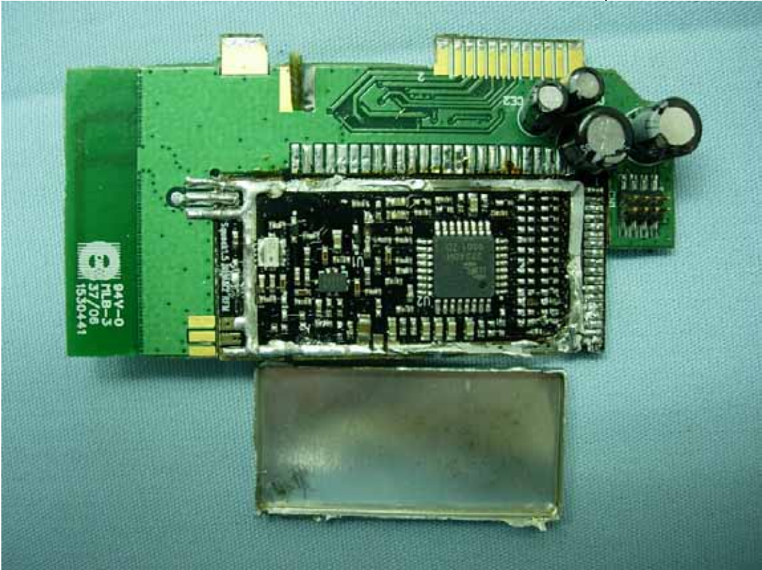
Figure 12 Internal View (RX Module, Back View)
