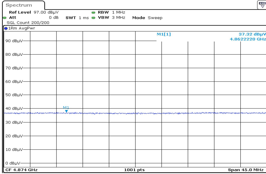
F2 X2 4874.0 Harmonic Vertical AVG
