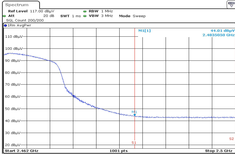
2462.0 F3 RestrictedBand Vertical AVG
