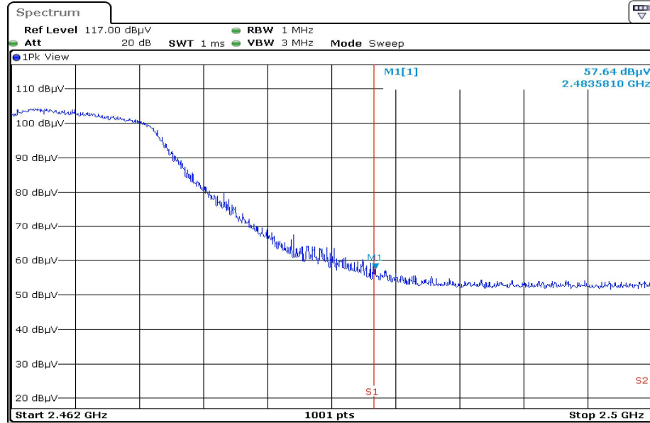
2462.0 F3 RestrictedBand Vertical PEAK
