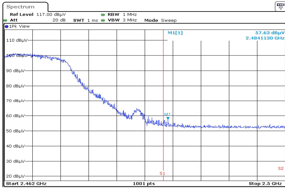
2462.0 F3 RestrictedBand Horizontal PEAK
