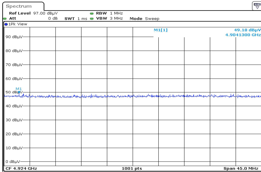
F3 X2 4924.0 Harmonic Horizontal PEAK
