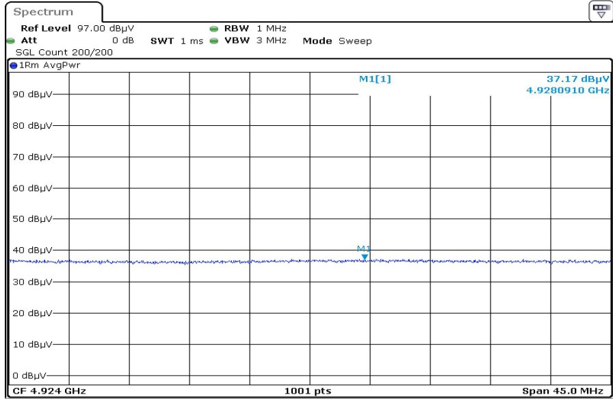
F3 X2 4924.0 Harmonic Vertical AVG
