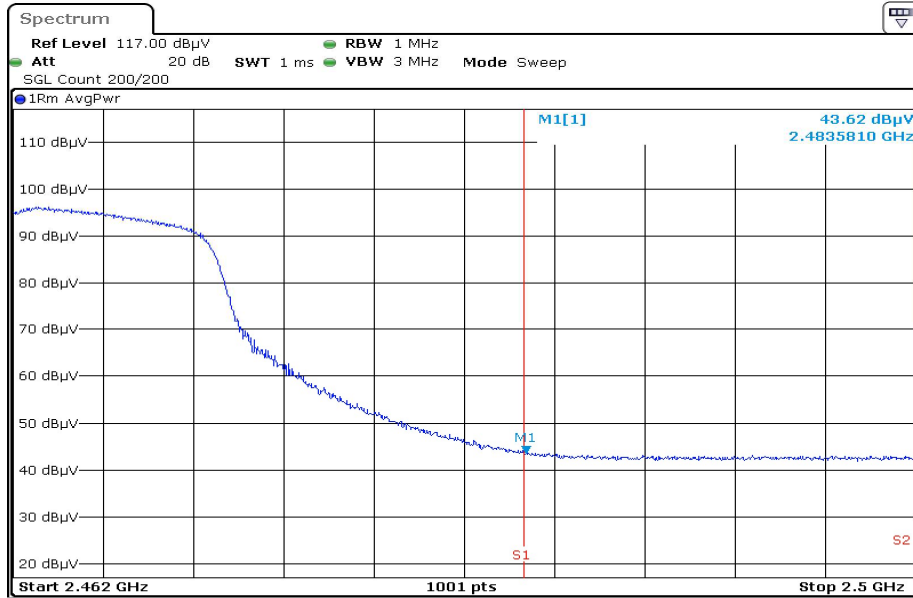
2462.0 F3 RestrictedBand Vertical AVG_1
