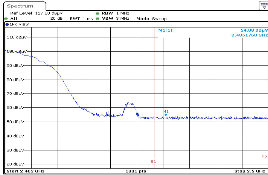
2462.0 F3 RestrictedBand Horizontal PEAK
