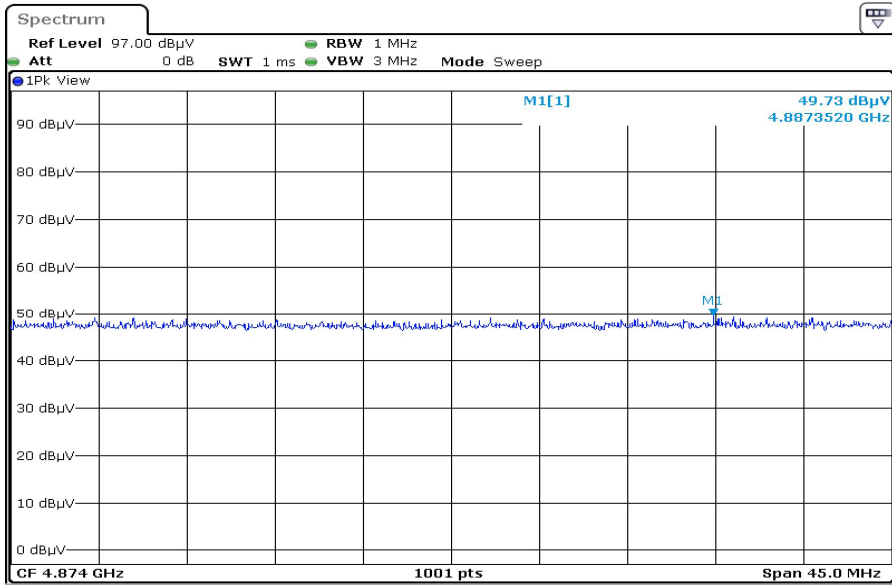
F2 X2 4874.0 Harmonic Vertical PEAK
