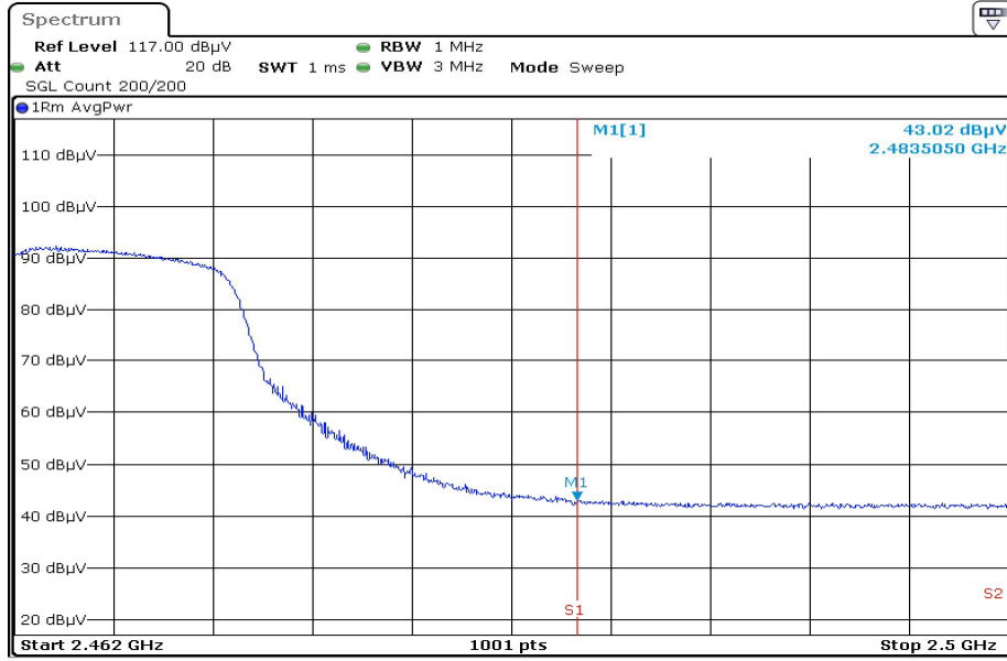
2462.0 F3 RestrictedBand Horizontal AVG
