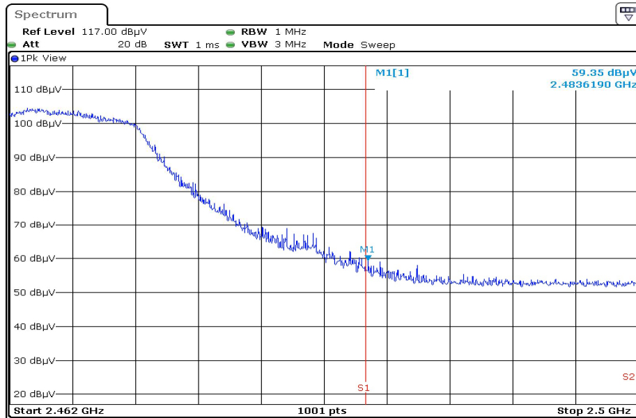
2462.0 F3 RestrictedBand Vertical PEAK_1
