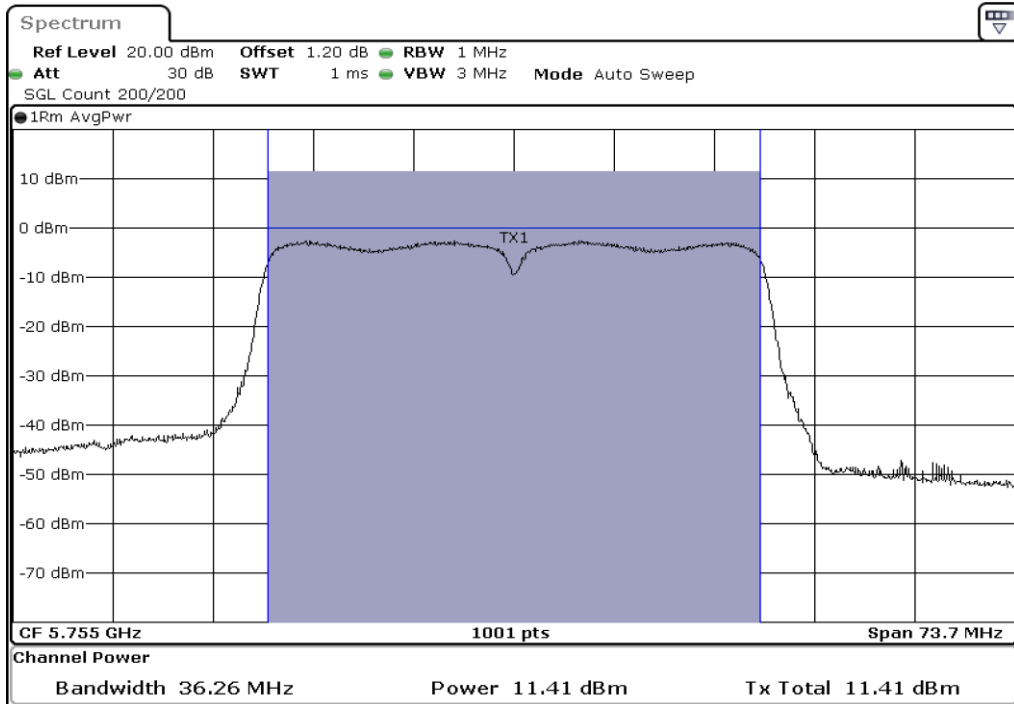
7 Output Power
