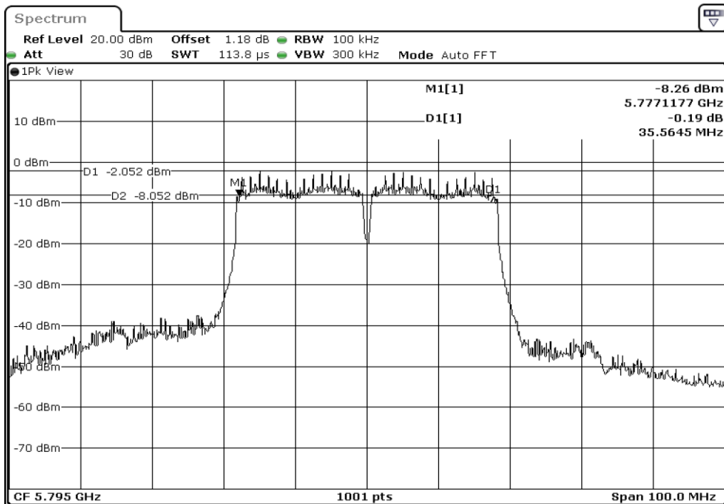
8 6dB Bandwidth
