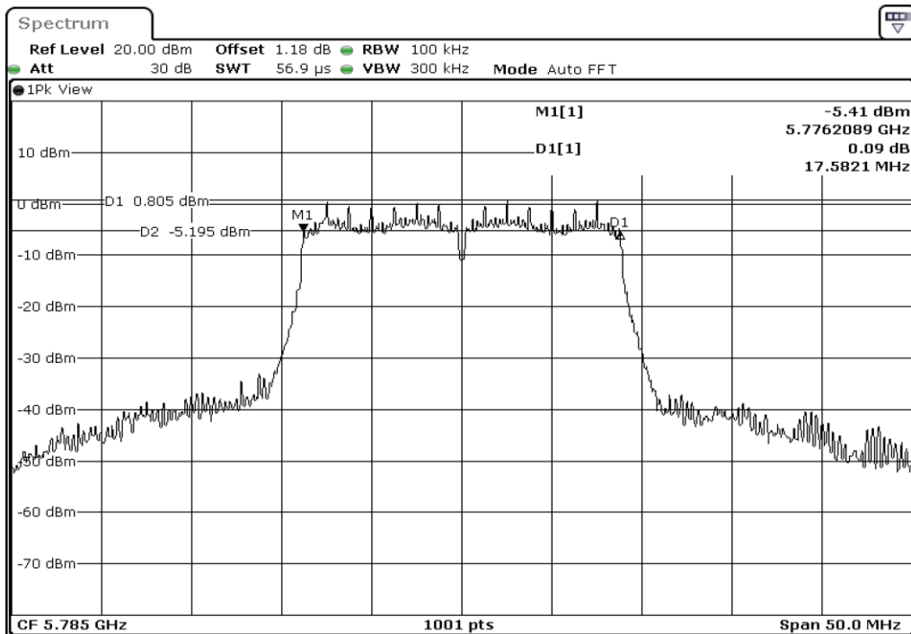
5 6dB Bandwidth
