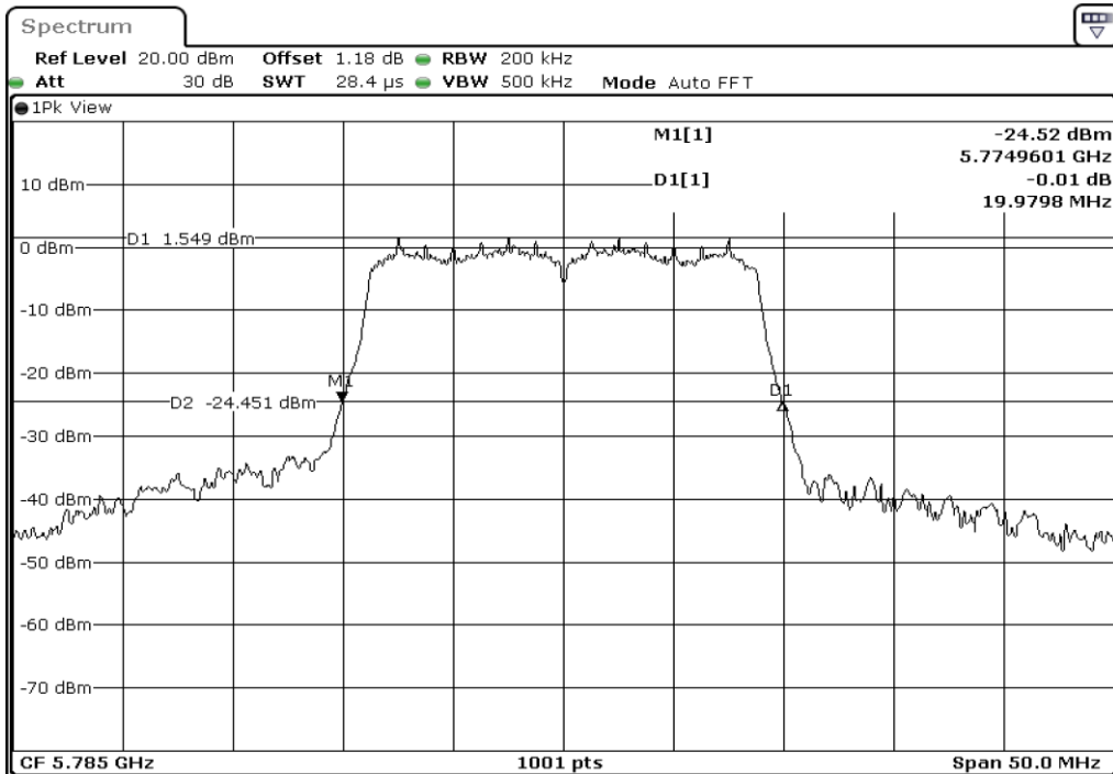
5 26dB Bandwidth
