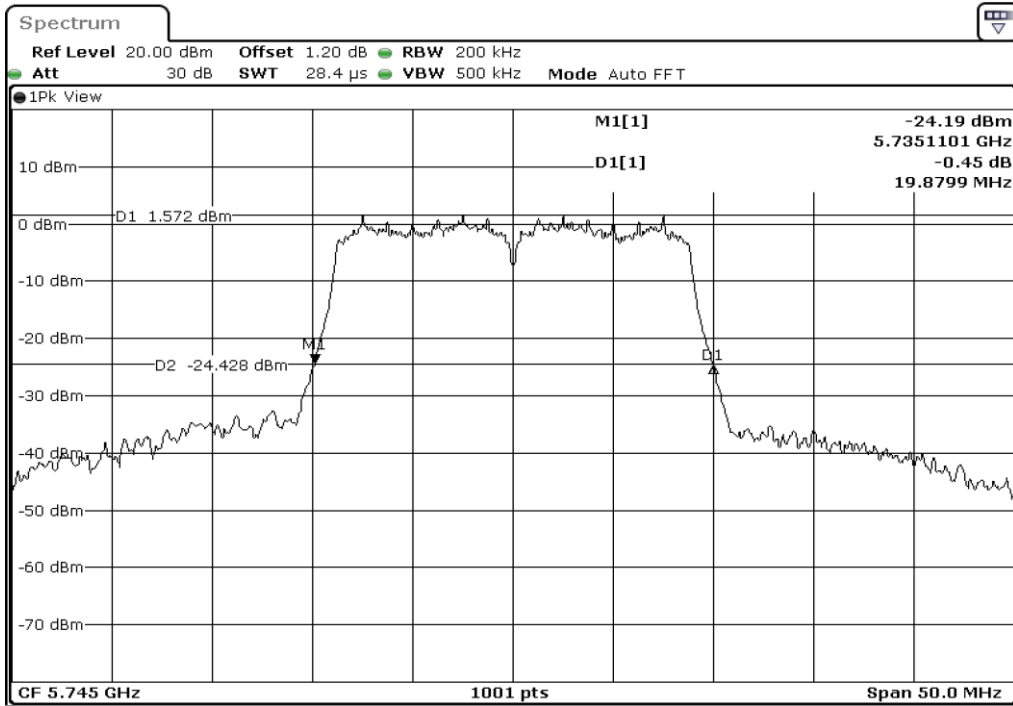
4 26dB Bandwidth
