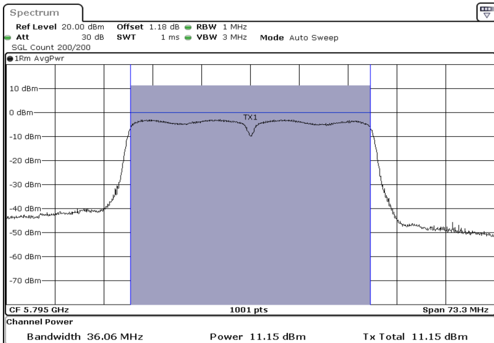
8 Output Power
