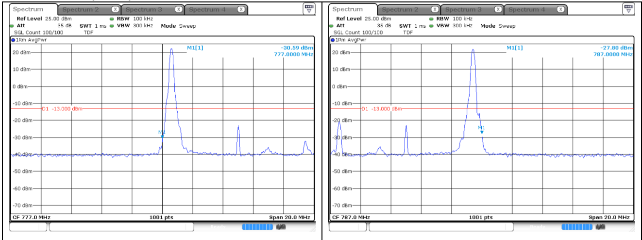
QPSK Middle Channel - 1 RB
