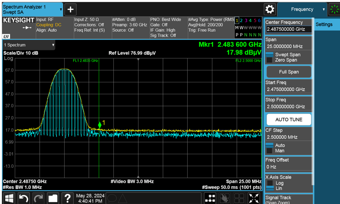
Radiated Restricted Band Edges plot – Peak Result (Ch.39, Y-V)
