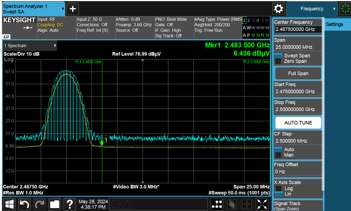
Radiated Restricted Band Edges plot – Average Result (Ch.39, Y-V)
