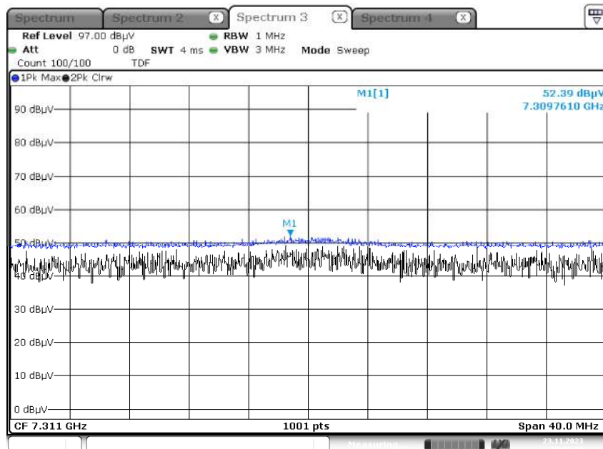
Radiated Spurious Emissions plot – Peak Result (802.11b_1 Mbps, Ch.6 3rd Harmonic)
