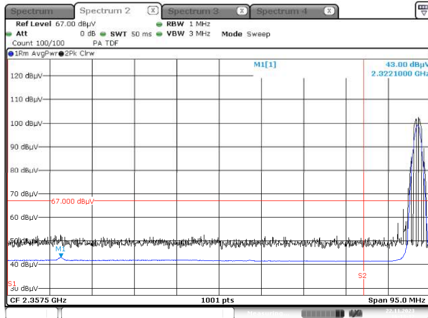
Radiated Restricted Band Edges plot – Average Result (Ch.0, Z-H)
