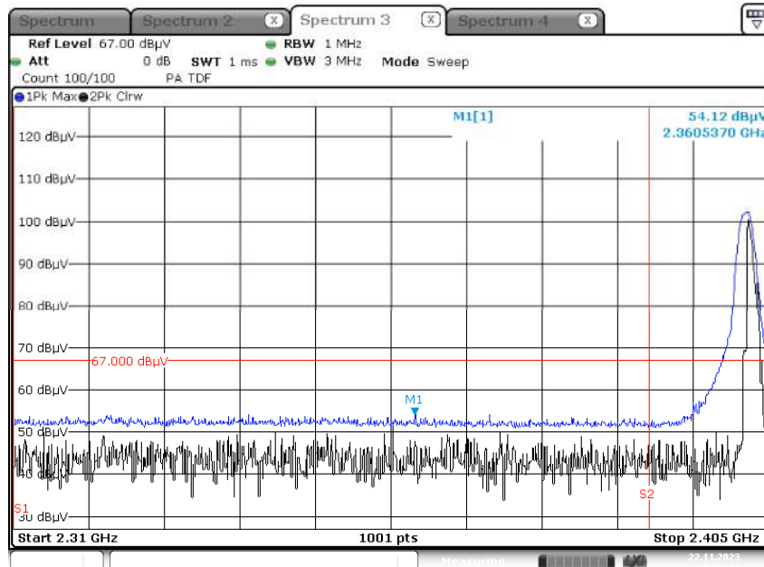
Radiated Restricted Band Edges plot – Peak Result (Ch.0, X-H)
