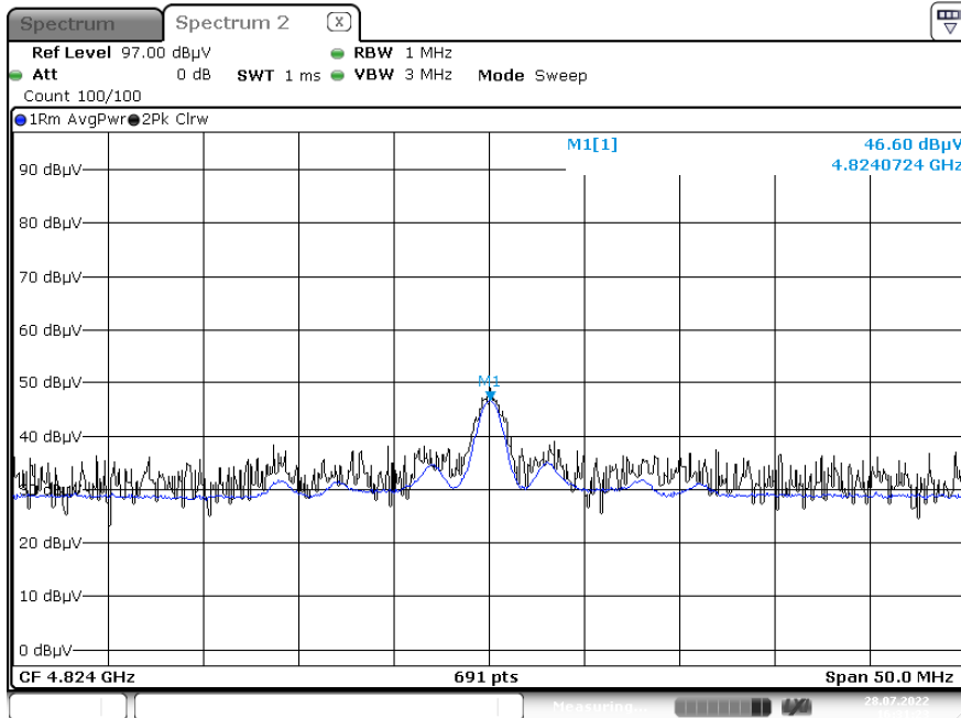
Radiated Spurious Emissions plot – Average Result (802.11b, Ch.1 2nd Harmonic)
