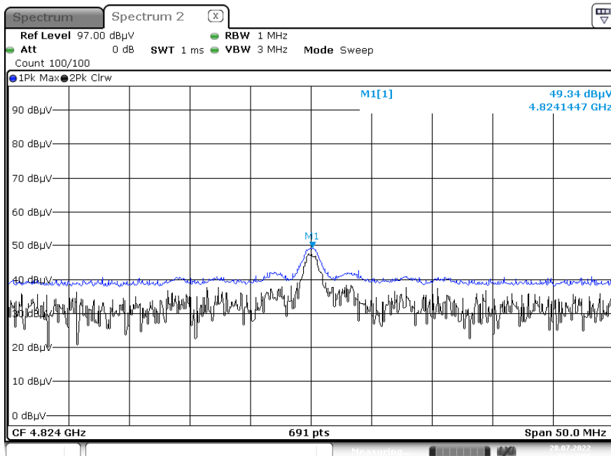
Radiated Spurious Emissions plot – Peak Result (802.11b, Ch.1 2nd Harmonic)
