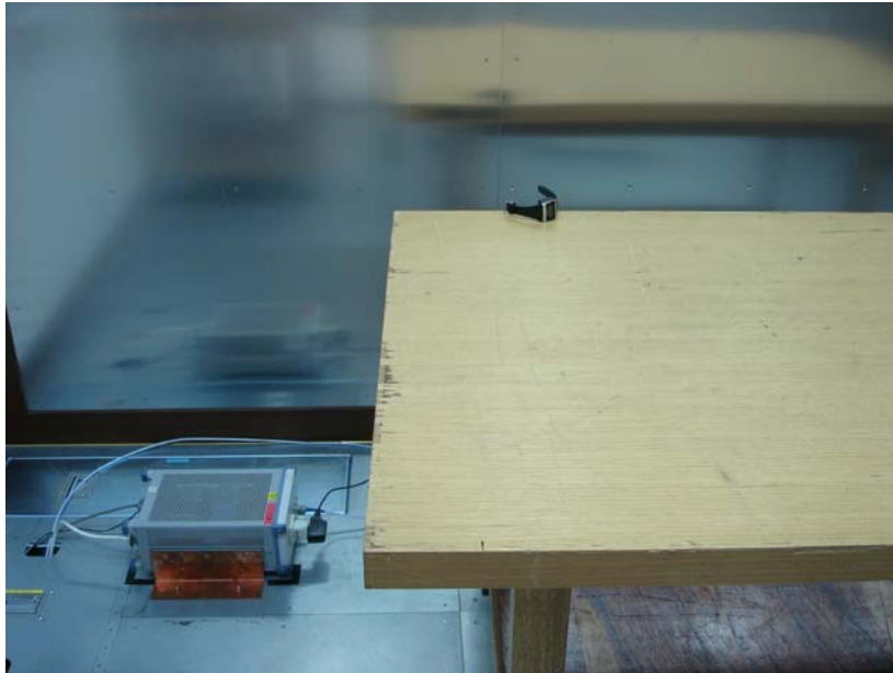
< Conducted emission >
