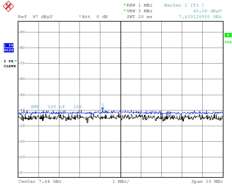
Radiated Spurious Emissions plot – Peak Result (Ch.39 3rd Harmonic, Y-V)
