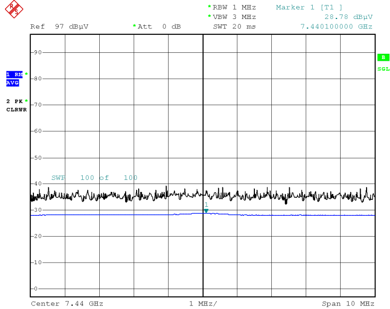
Radiated Spurious Emissions plot – Average Result (Ch.39 3rd Harmonic, Y-V)
