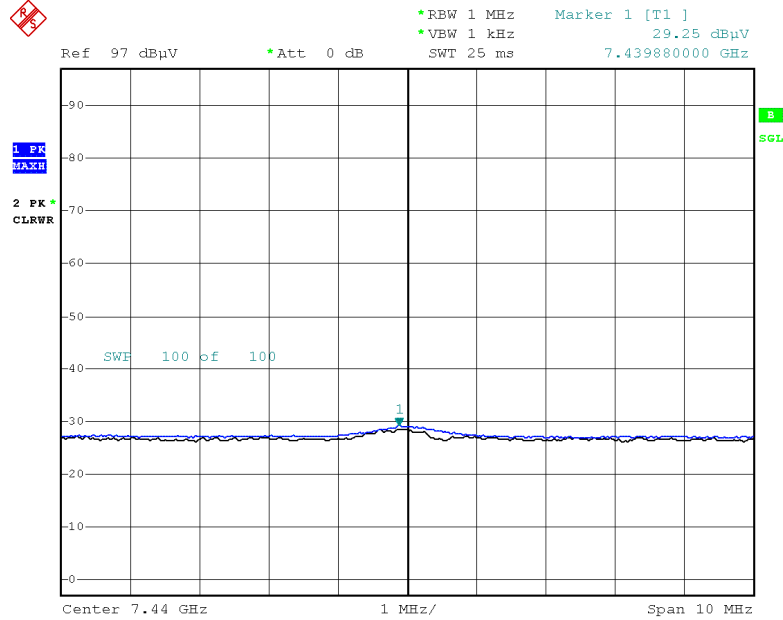
Radiated Spurious Emissions plot – Average Result, V 3rd
