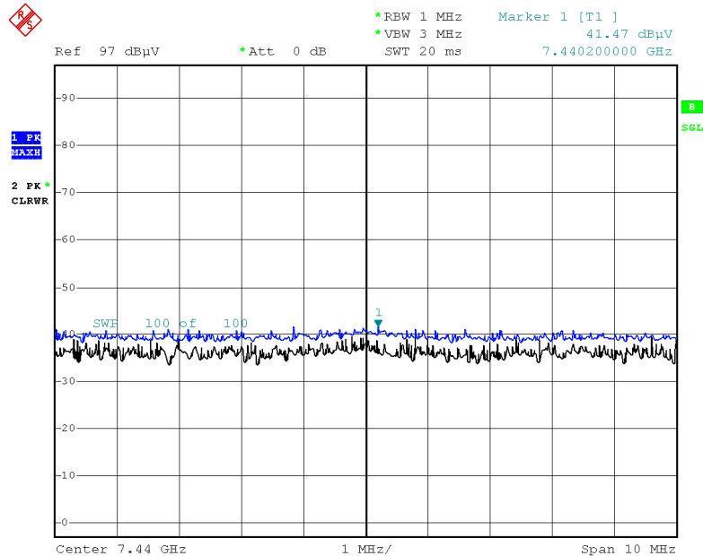
Radiated Spurious Emissions plot – Peak Result, V 3rd
