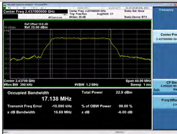
99 % Bandwidth plot (802.11n_HT20-CH 6)
