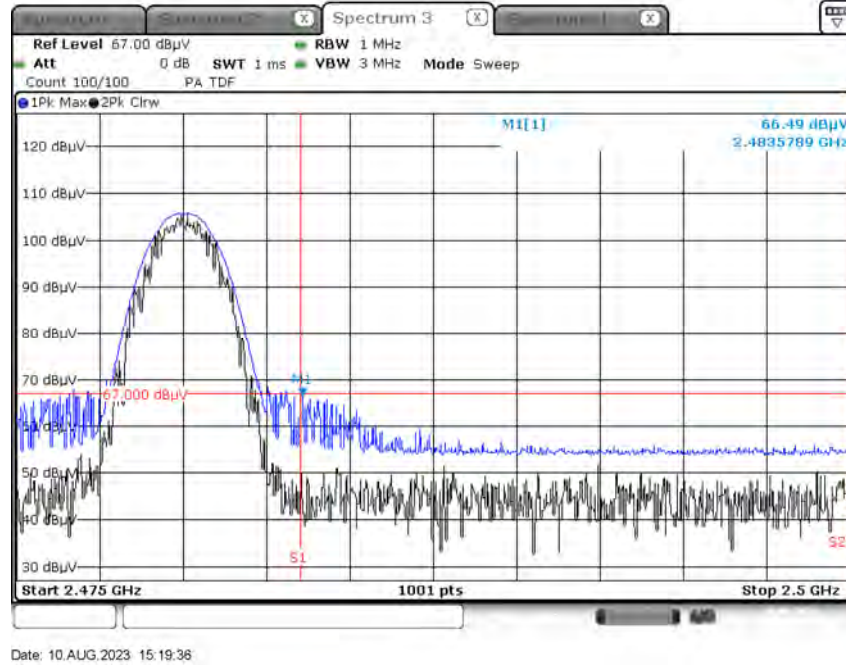
Radiated Restricted Band Edges plot – Average & Peak Result ( \pi/4 DQPSK, Ch.78, Z-V)
