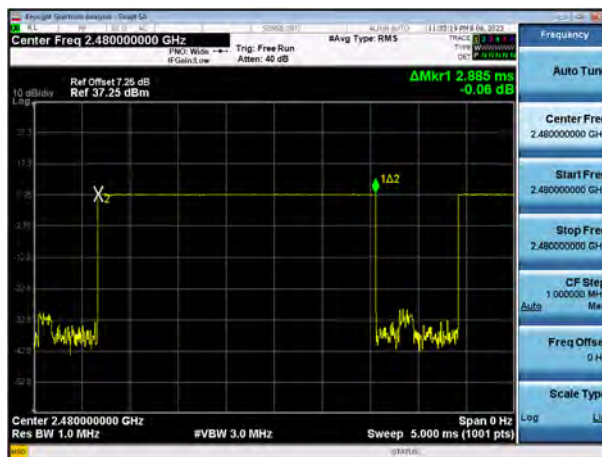
Test Plots (GFSK) Dwell Time (CH.78)
