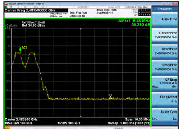
8DPSK(with hopping) Band Edge(CH.78)
