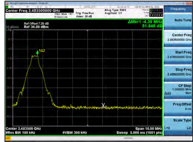
8DPSK(without hopping) Band Edge(CH.78)
