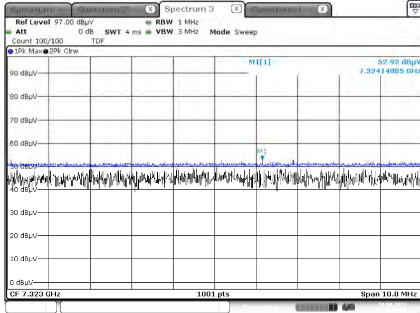
Radiated Spurious Emissions plot – Average & Peak Result (8DPSK, Ch39 3rd Harmonic, H)
