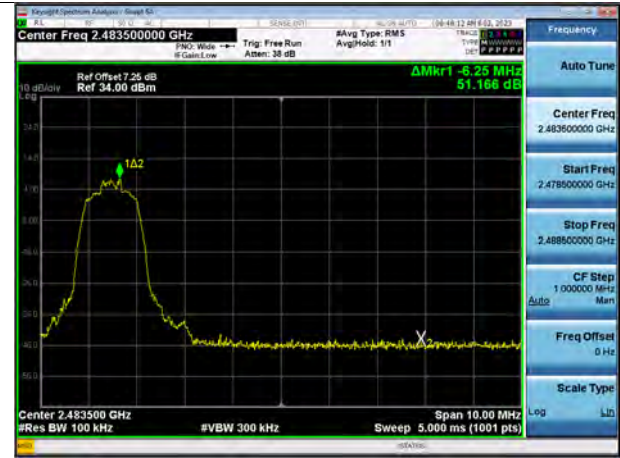
\pi/4 DQPSK (without hopping) Band Edge(CH.78)
