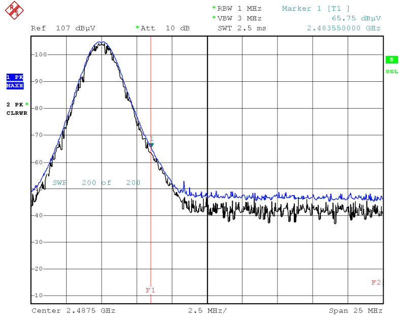
Radiated Restricted Band Edges plot – Average & Peak Result ( \pi/4 DQPSK, Ch.78, V)
