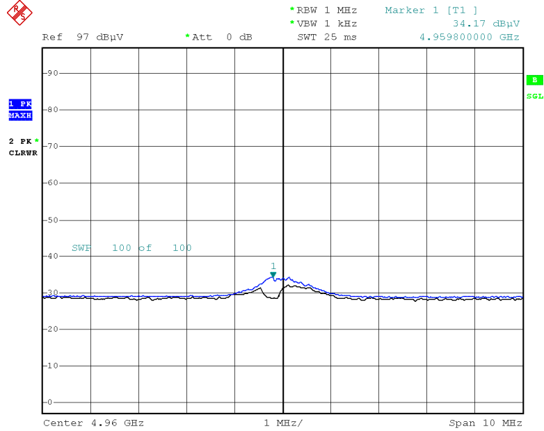
Radiated Spurious Emissions plot – Average Result (GFSK, Ch.78 2nd Harmonic, V)
