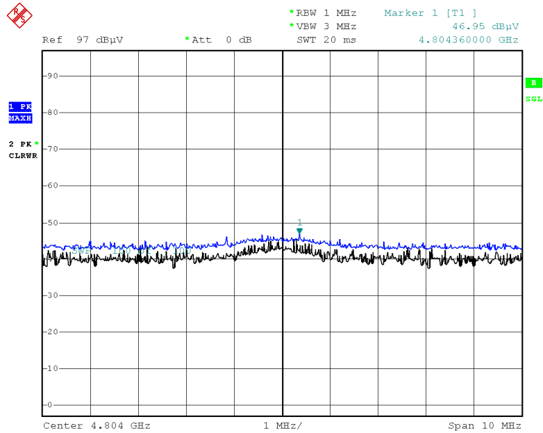
Radiated Spurious Emissions plot – Peak Result (GFSK, Ch.0 2nd Harmonic, Y-V)
