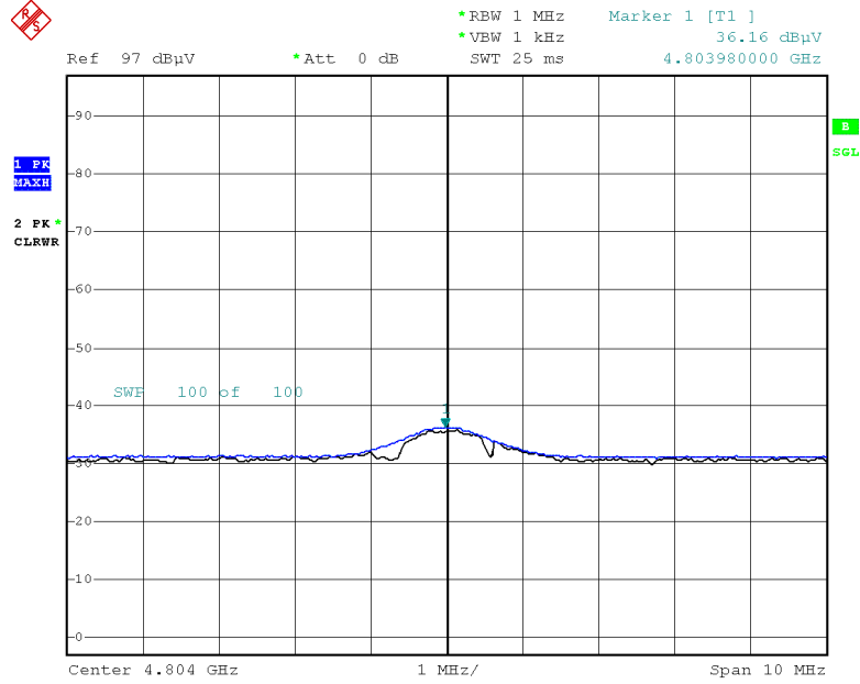
Radiated Spurious Emissions plot – Average Result (GFSK, Ch.0 2nd Harmonic, Y-V)
