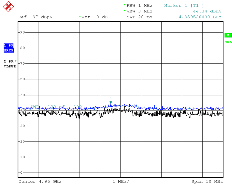
Radiated Spurious Emissions plot – Peak Result (GFSK, Ch.78 2nd Harmonic, V)
