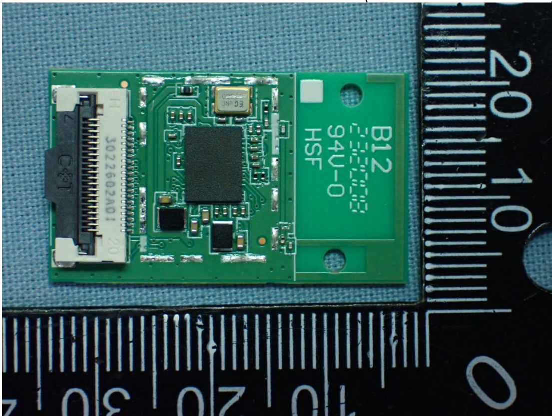
Figure 7 Internal View (Removed Shielded Cover)
