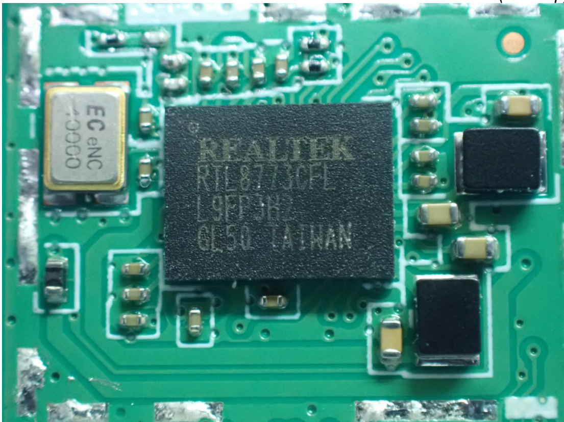
Figure 8 Internal View (RF Chip)
