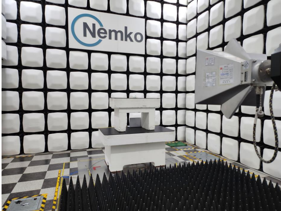
Radiated Test_Above 1 GHz_Rear
