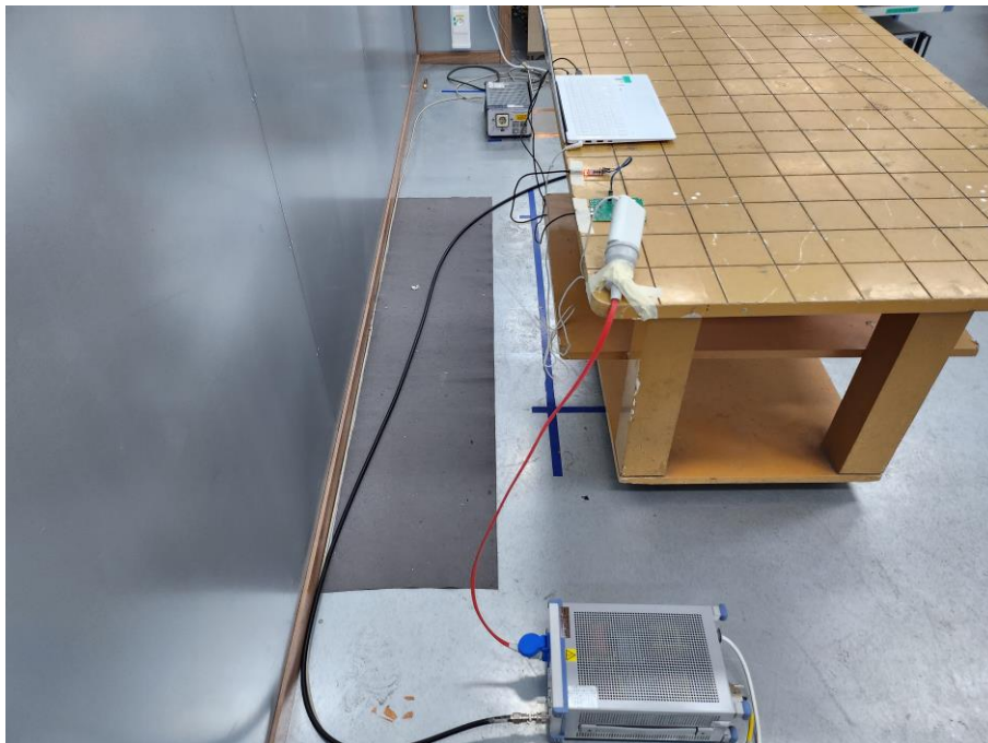
AC Line Conducted Test_Rear
