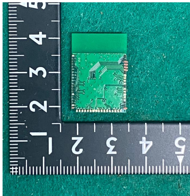
Rear View of Main Board
