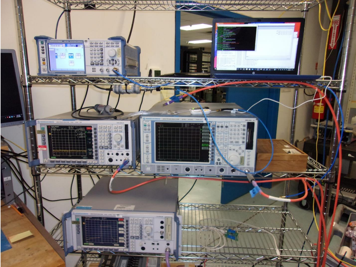
Conducted Antenna Port
