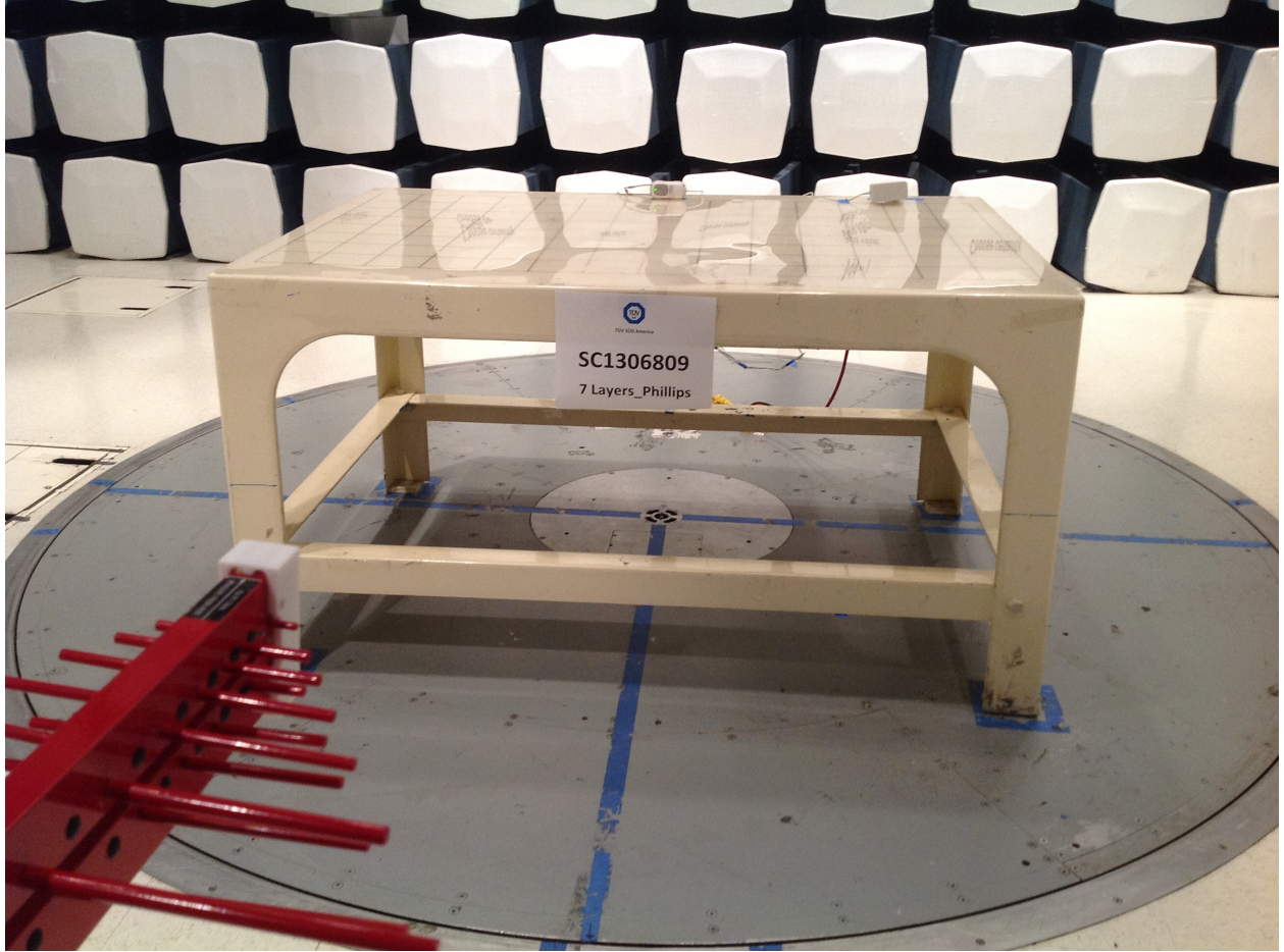
Radiated Emissions Test Setup (30-1GHZ)
