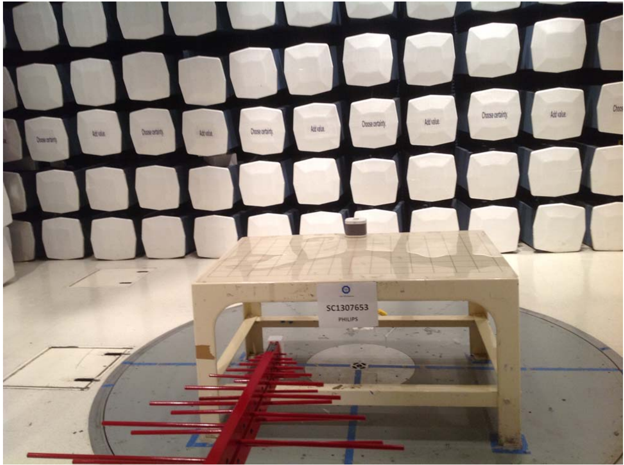
Radiated Emissions Test Setup (30-1GHZ) /Band Edges/OBW
