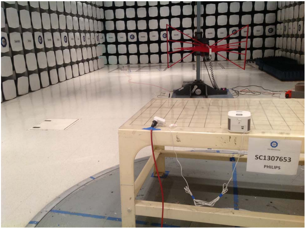
Radiated Emissions Test Setup RX Mode"Back Side" (30-1GHZ)
