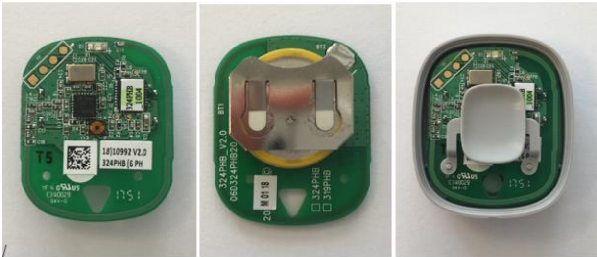
Figure 2: 324PHB/324PHW: PCBA top side (left), bottom side (middle) and PCBA assembled in enclosure bottom part (right).
