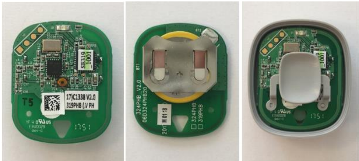
Figure 2: 319PHB/319PHW: PCBA top side (left), bottom side (middle) and PCBA assembled in enclosure bottom part (right).
