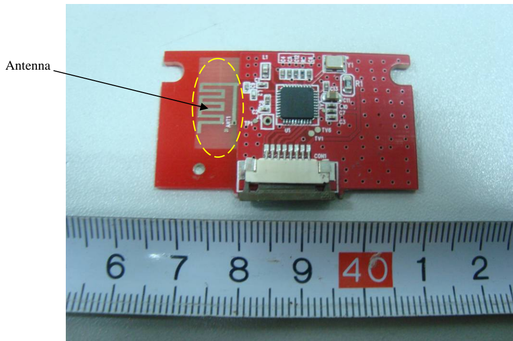
EUT – RF Board Top View
