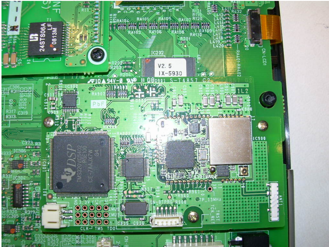
Internal View of the IX-5930 Showing IX-59BTINF Placement
