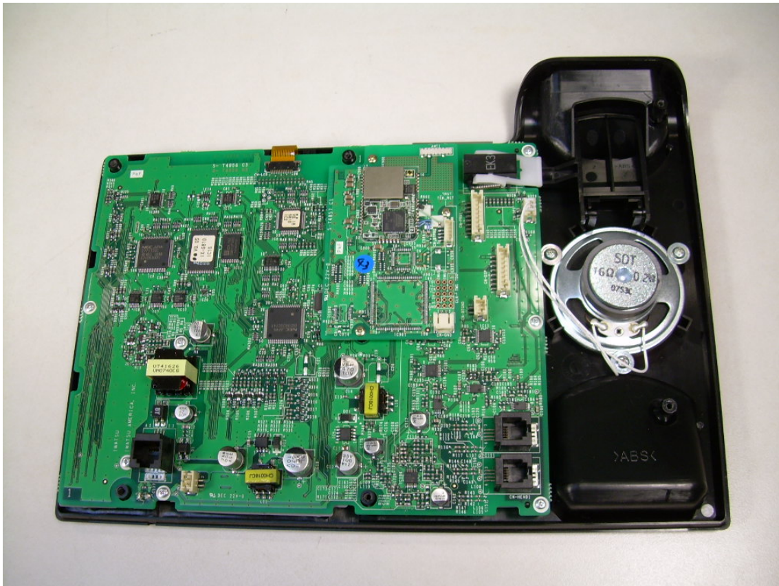
Internal View of the IX-5810 Showing IX-58BTINF Placement
