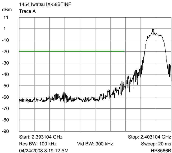
Trace A Channel 0, bandedge plot
