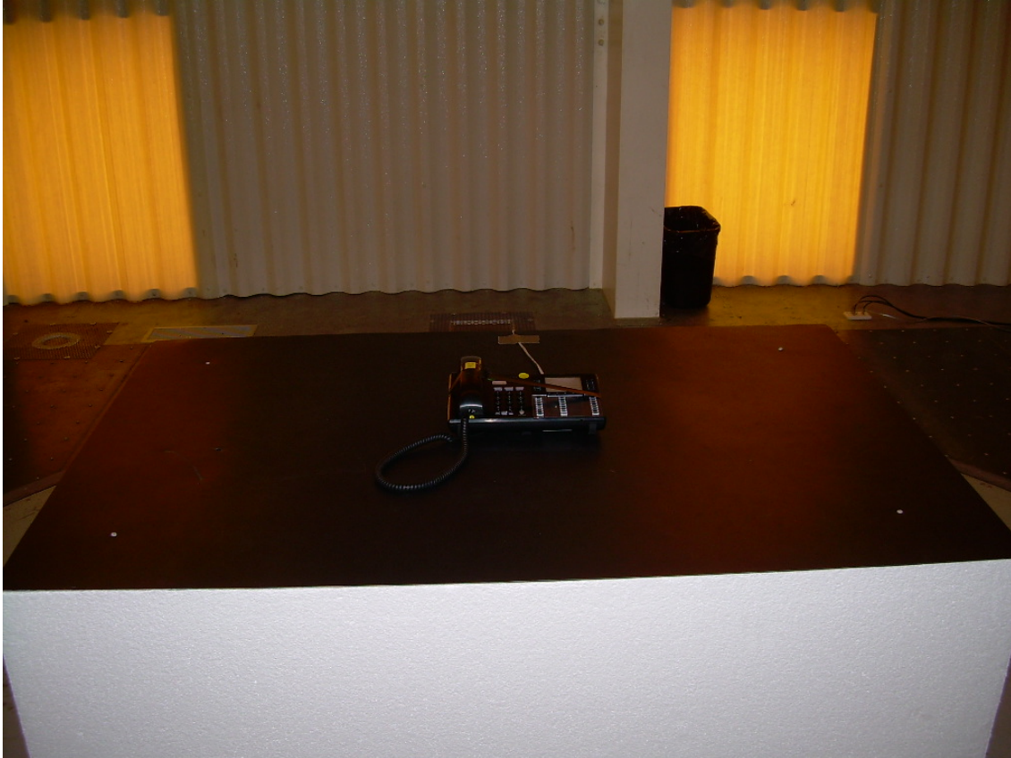
Photograph 4 - Front View Radiated Spurious Emissions Configuration - Horizontal Placement
