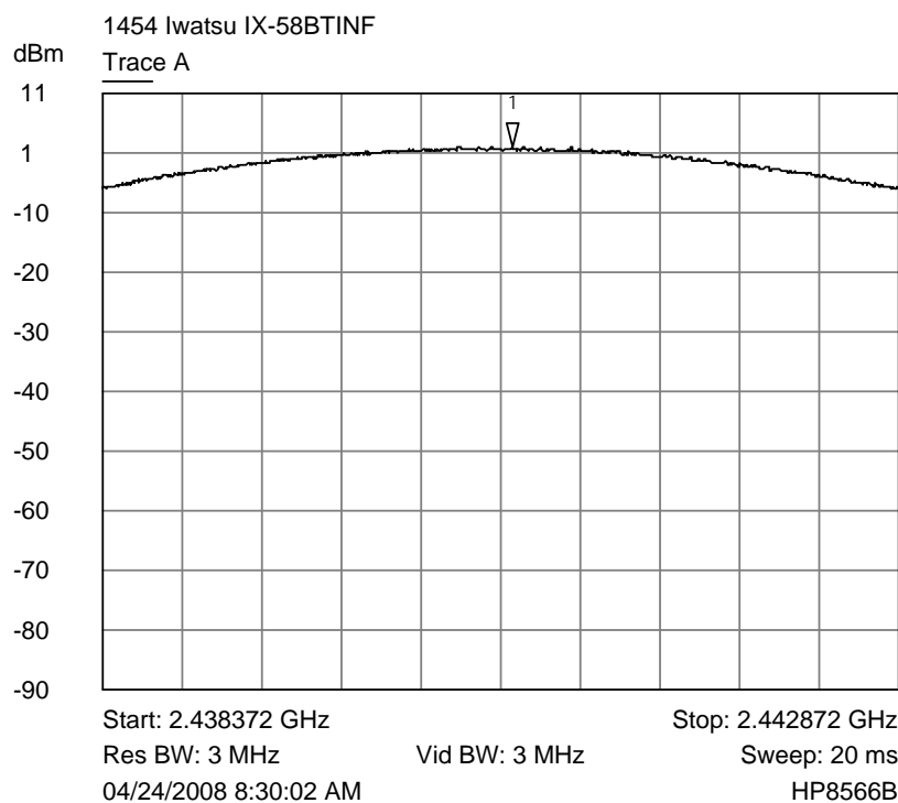
Trace A Channel 39, output power plot
