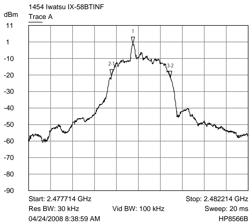
Trace A Channel 78, band width plot
