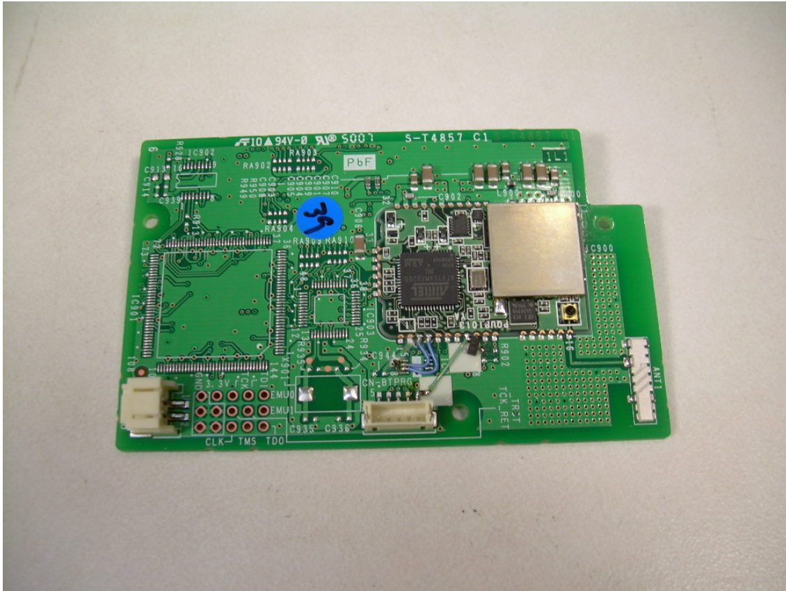
Photograph 8 - Component Side of the IX-58BTINF
