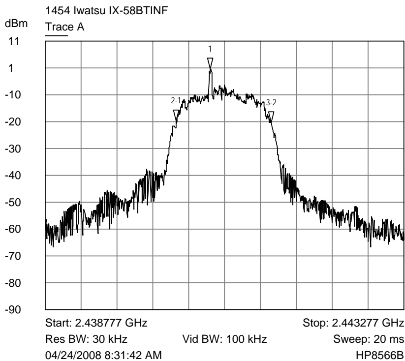
Trace A Channel 39, bandwidth plot
