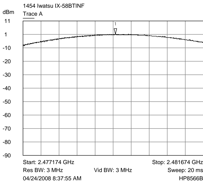
Trace A Channel 78, output power plot
