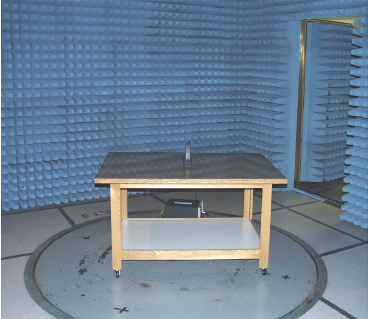
Front View of Worst Case Radiated and Line Conducted Emissions Test Set-up
