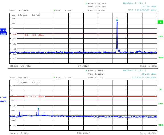
Figure 8.2-2: 1.4 MHz LTE QPSK 30 MHz – 8 GHz
