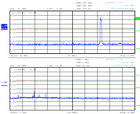
Figure 8.2-6: 5 MHz LTE QPSK 30 MHz – 8 GHz
