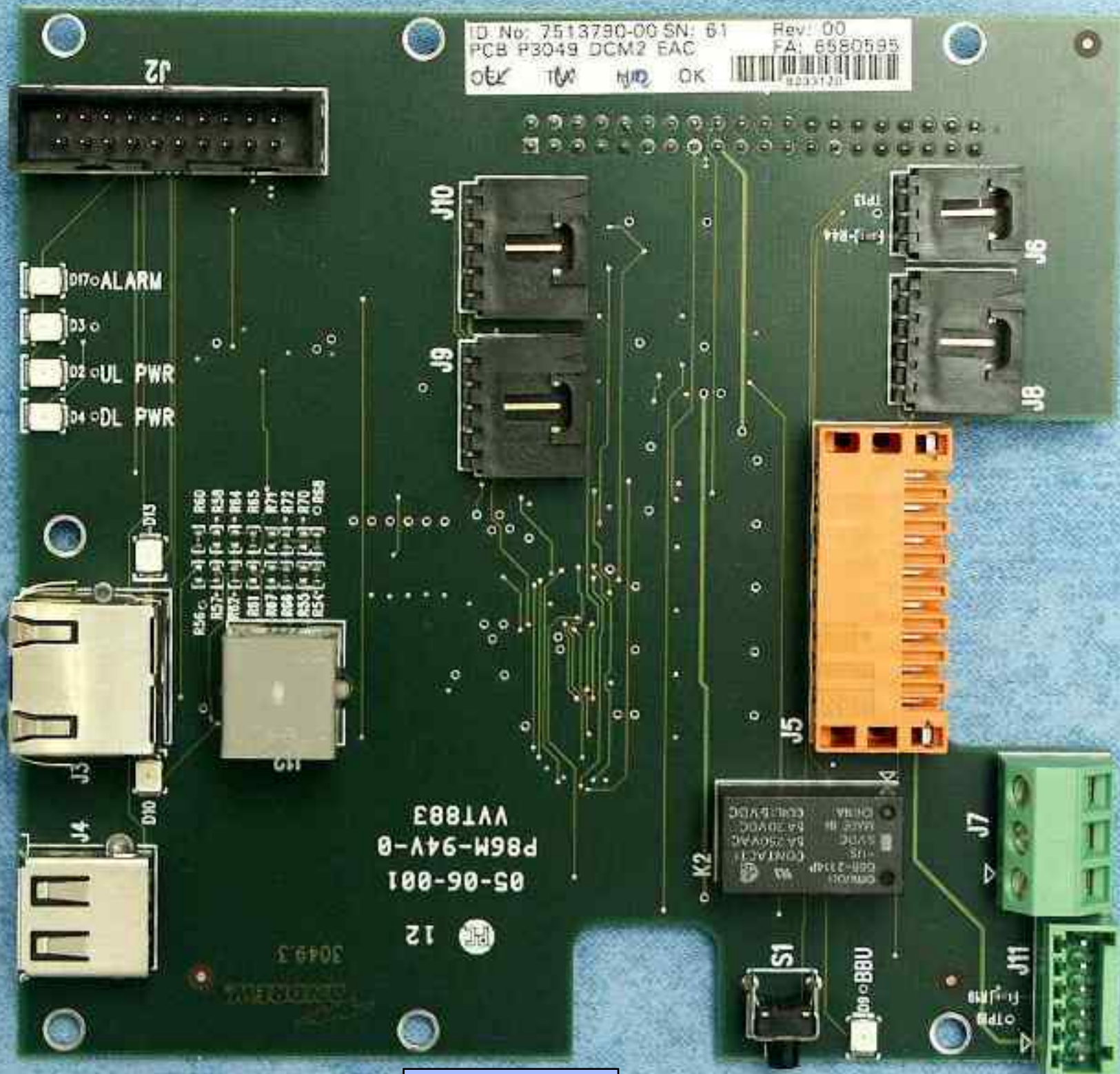
EAC - Controller Card Top
