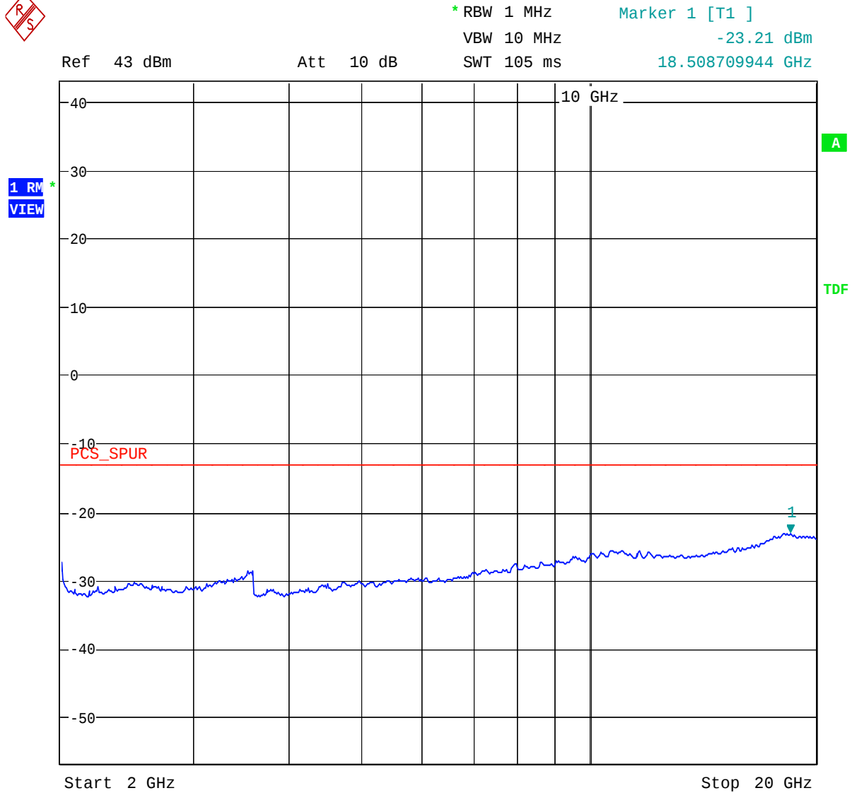
Figure 18- Antenna Conducted Spurious- Downlink – IS-95 – Channel 600
