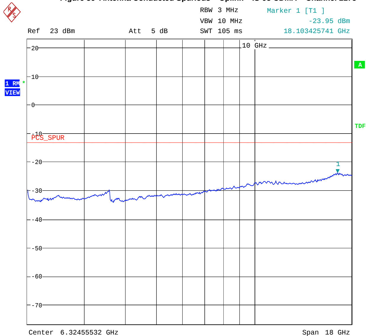
Figure 36 Antenna Conducted Spurious – Uplink – IS-95 CDMA – Channel 1175
