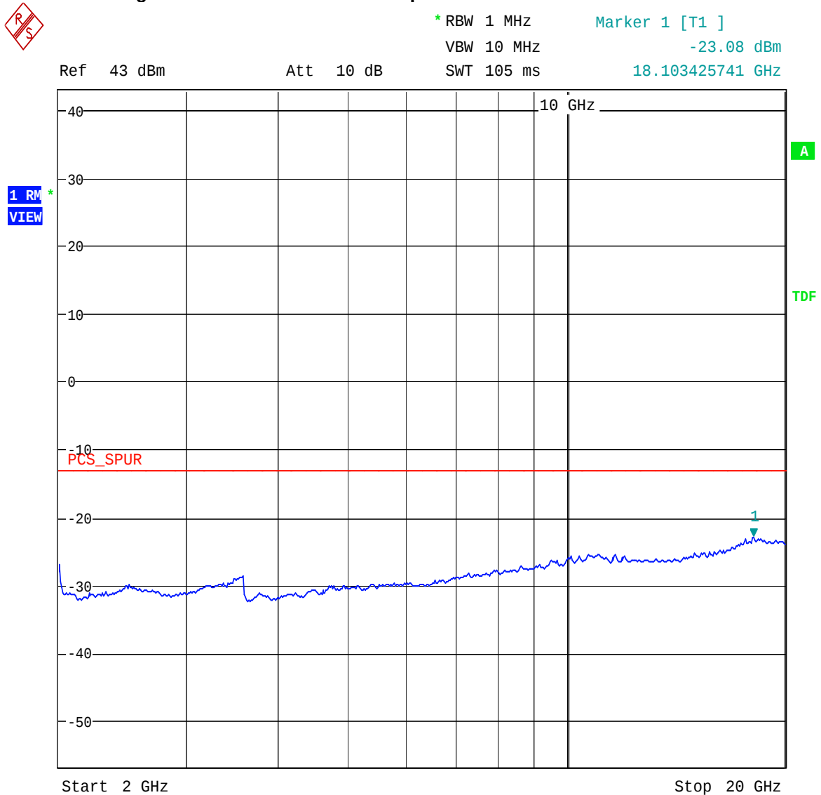
Figure 21- Antenna Conducted Spurious- Downlink – IS-95 – Channel 1175
