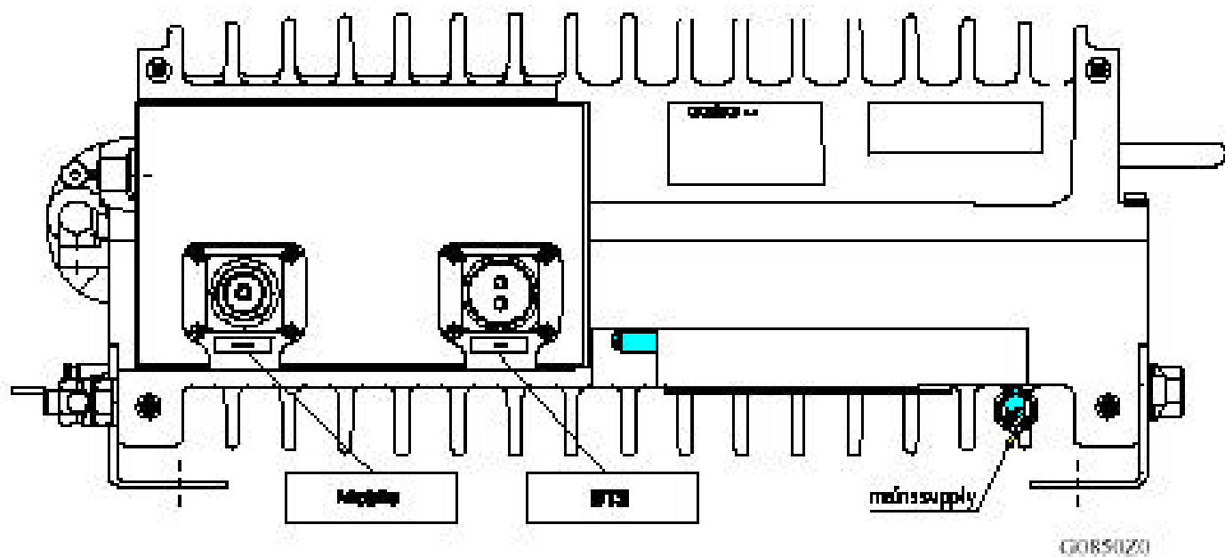
END VIEW SHOWING RF & OPTICAL CONNECTIONS
