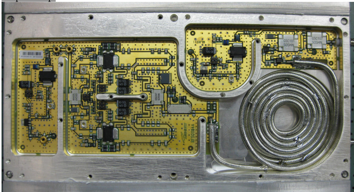
Amplifier top:
