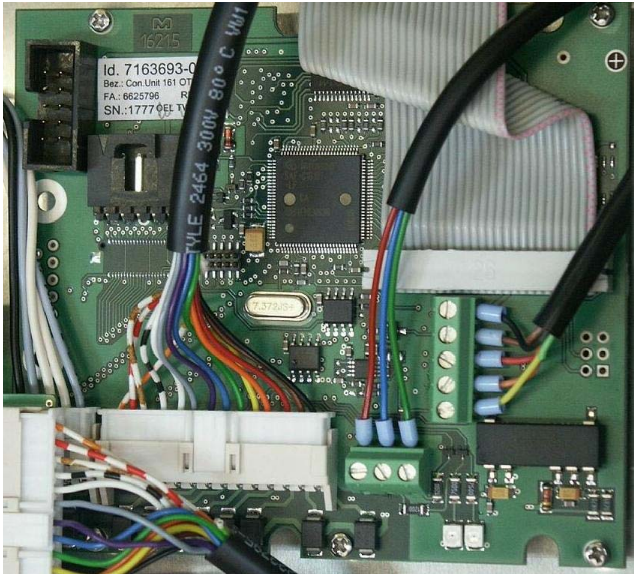
Control Board
