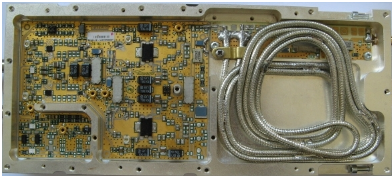
PA 850 MHz - Bottom
