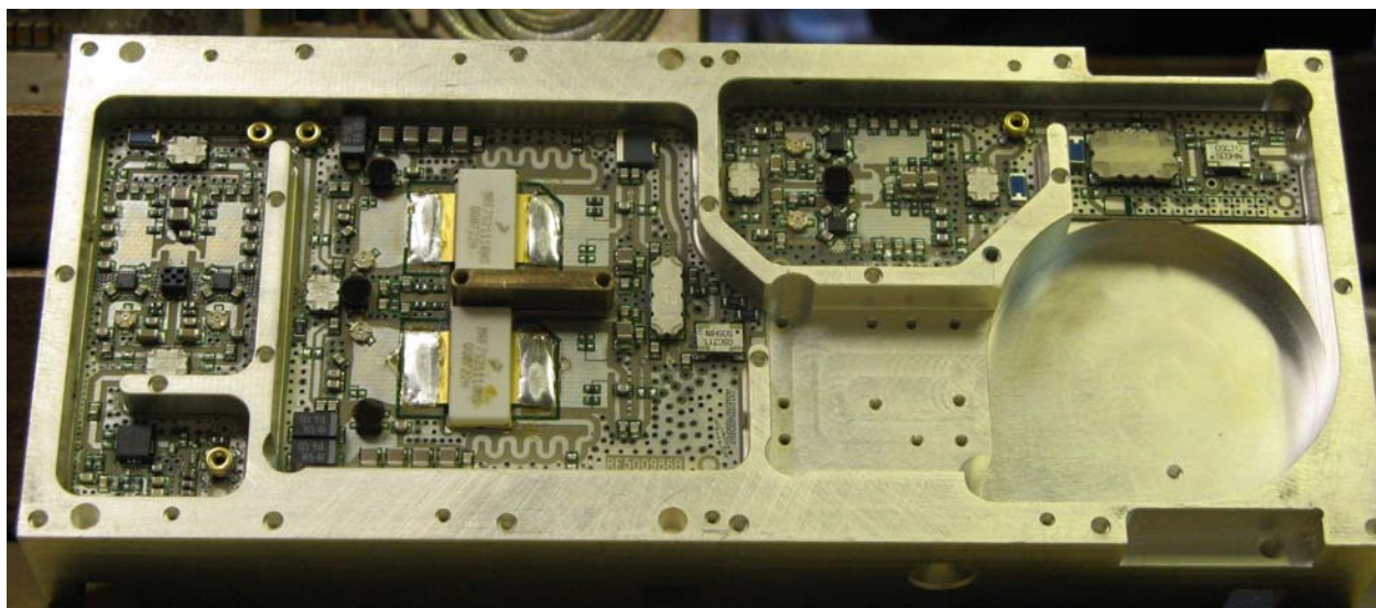
1900 MHz PA – Top
