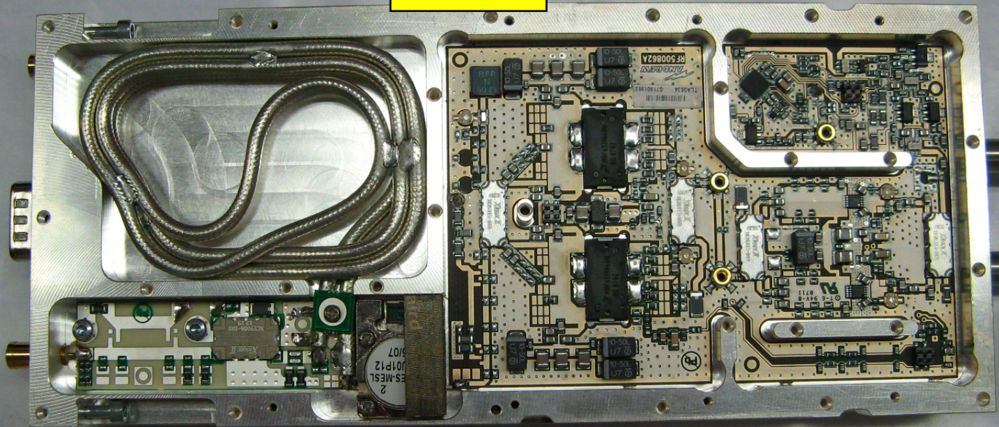
2100 MHz rf board
